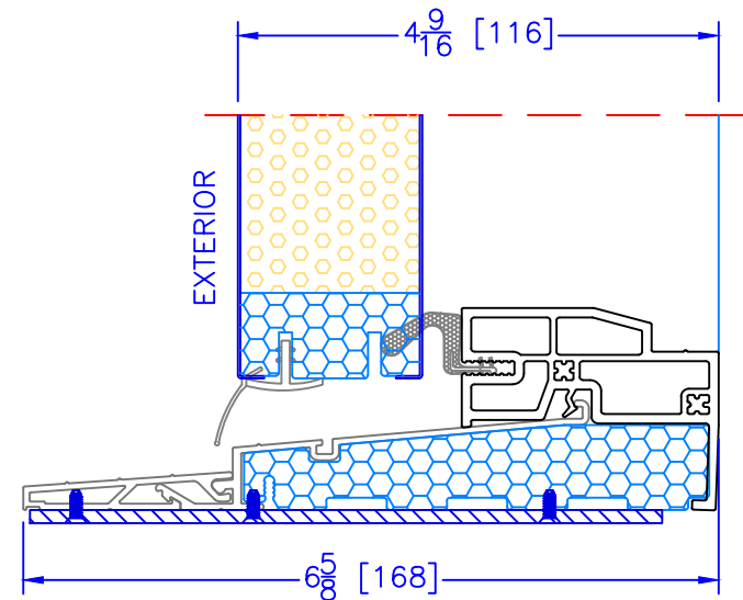
4 \frac{9}{16} " OUTSWING HIGH PERFORMANCE SILL 2 PC ALUMINUM (2" EXT) (USED WITH ALL OTHER EXTERIOR OPTIONS)
