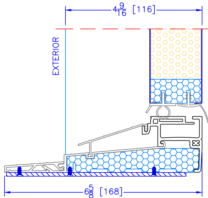
4 \frac{9}{16} " INSWING HIGH PERFORMANCE SILL 2 PC ALUMINUM (2" EXT) (USED WITH ALL OTHER EXTERIOR OPTIONS)
