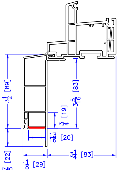
FLUSH EXTENSION (OFFERED WITH AND WITHOUT NAILING FIN)
