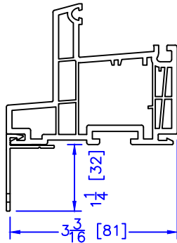
FLASHING FLANGE
