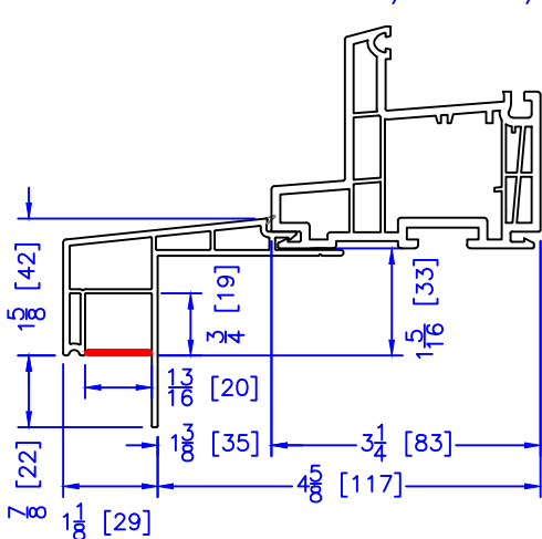
1-1/2" x 1-3/8" EXTENDED BM/J-TRIM
