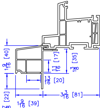
3-1/2" BM/J-TRIM
