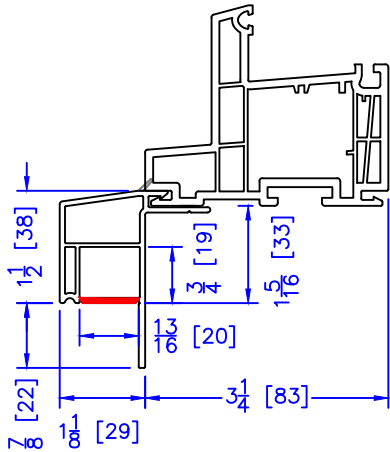
2" 180 BM/J-TRIM
