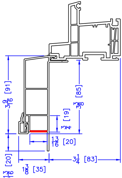
3-1/2" 180 BM/J-TRIM
