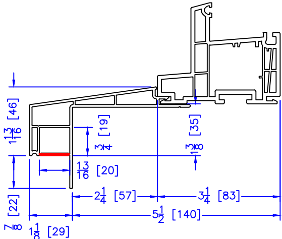
1-1/2" x 2-1/4" EXTENDED BM/J-TRIM *RESIDENTIAL APPLICATION ONLY*
