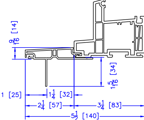
FLUSH EXTENSION (OFFERED WITH AND WITHOUT NAILING FIN)
