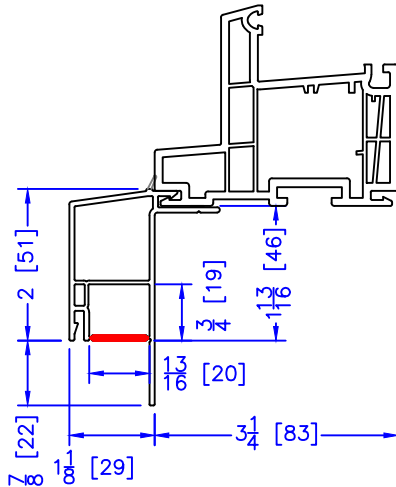
2" BM/J-TRIM
