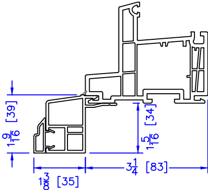
1-1/2" RENO BM
