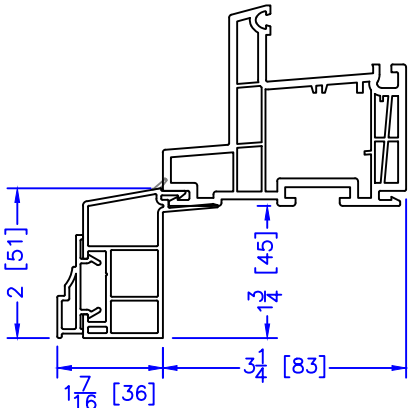
2" RENO BM
