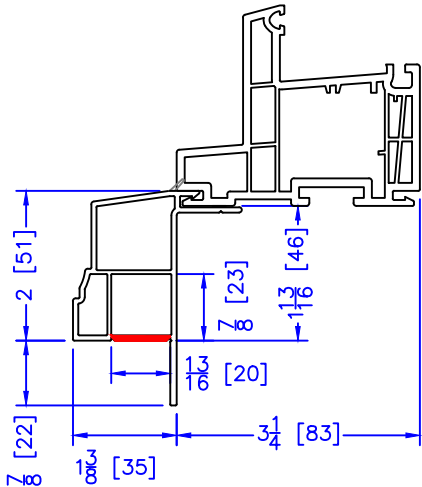
2" 180 BM/J-TRIM
