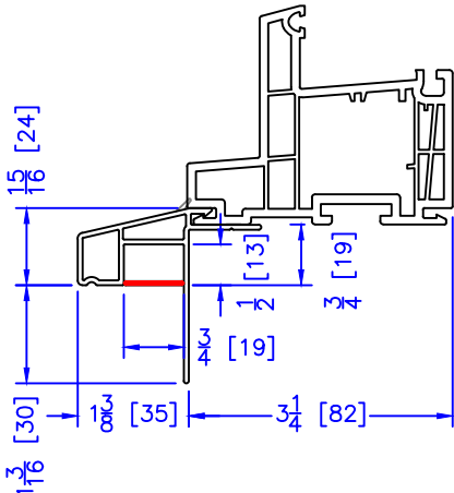
3-1/2" 180 BM/J-TRIM
