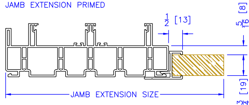
JAMB EXTENSION PRIMED
