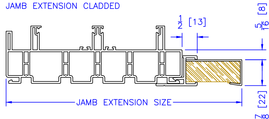
JAMB EXTENSION CLADDED
