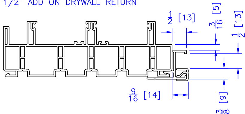
1/2" ADD ON DRYWALL RETURN
