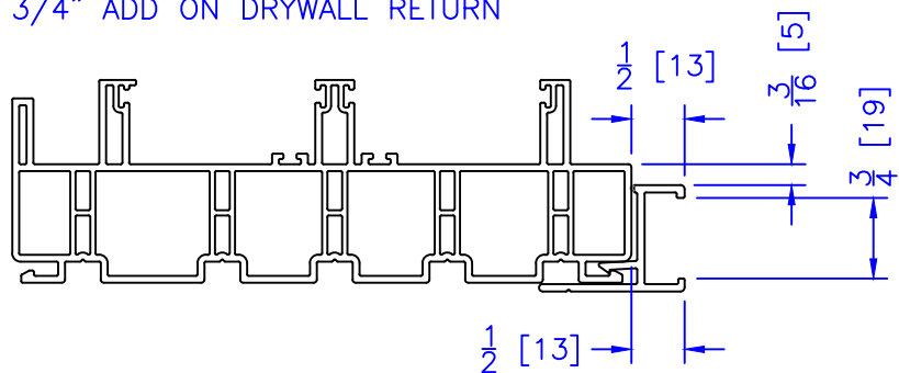
3/4" ADD ON DRYWALL RETURN
