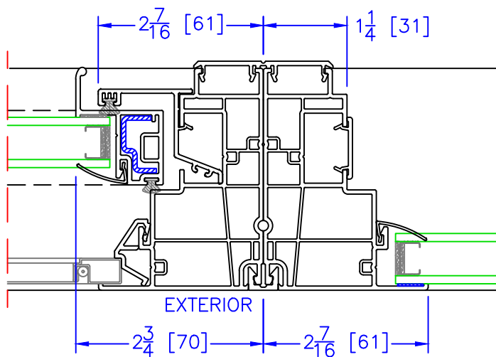
OPERATOR/FIXED VERTICAL MULLION
