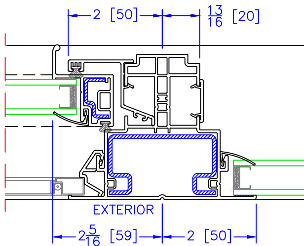
OPERATOR/FIXED VERTICAL T-MULLION
