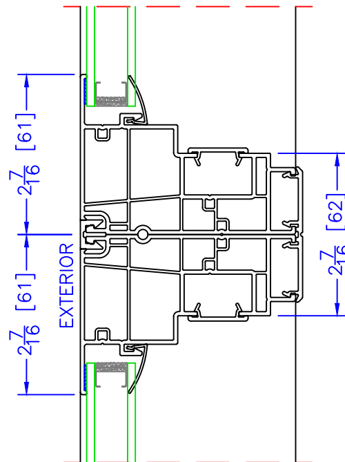
FIXED/FIXED HORIZONTAL MULLION
