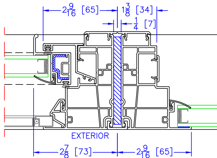
OPERATOR/FIXED VERTICAL REINFORCEMENT MULLION
