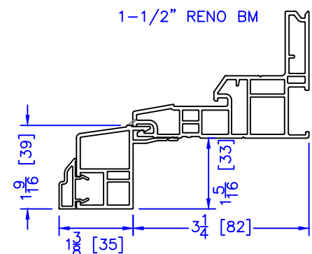
1-1/2" RENO BM
