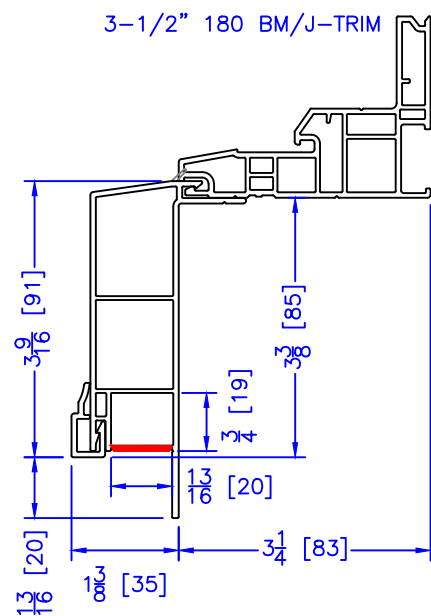
3-1/2" 180 BM/J-TRIM
