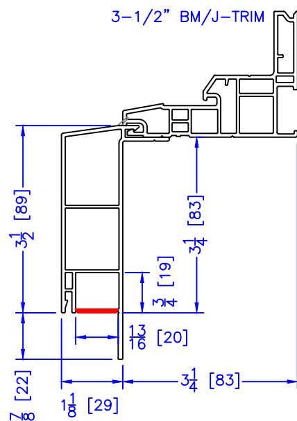
3-1/2" BM/J-TRIM
