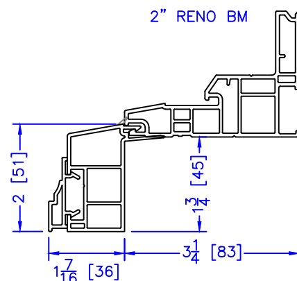
2" RENO BM
