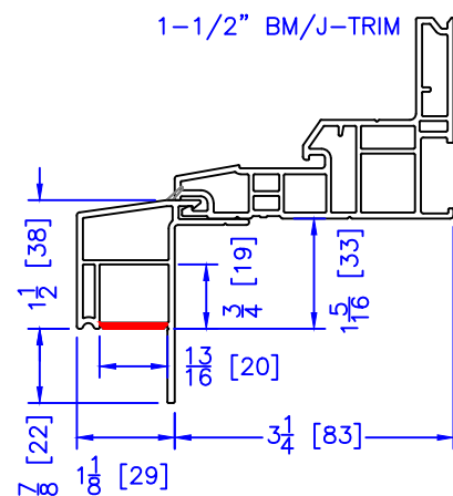
1-1/2" BM/J-TRIM
