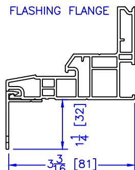
FLASHING FLANGE
