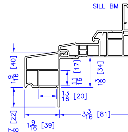
2" BM/J-TRIM
