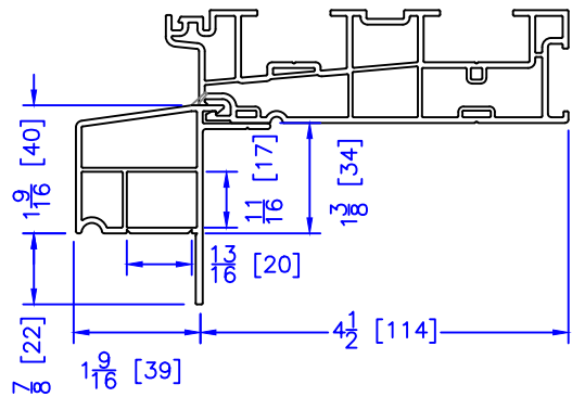
SILL BM
