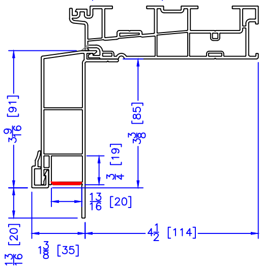
3-1/2" 180 BM/J-TRIM
