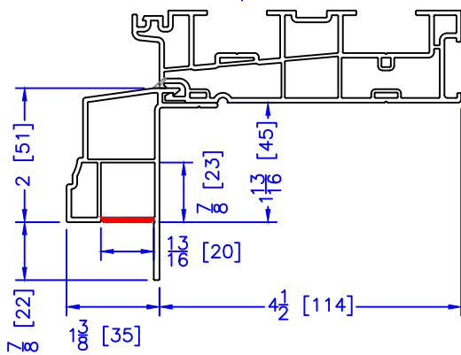
2" 180 BM/J-TRIM
