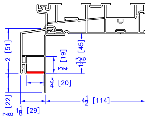
2" BM/J-TRIM
