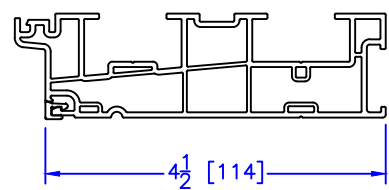
EXTERIOR ACCESSORY GROOVE CLOSEOUT
