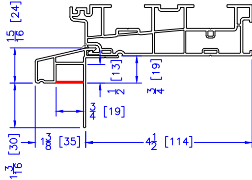
7/8" BM/J-TRIM
