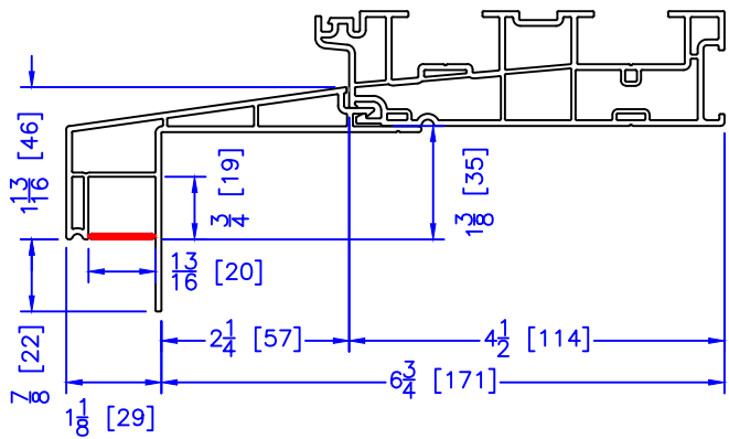
1-1/2" x 2-1/4" EXTENDED BM/J-TRIM *RESIDENTIAL APPLICATION ONLY*
