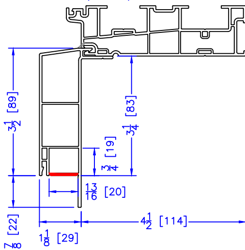
3-1/2" BM/J-TRIM
