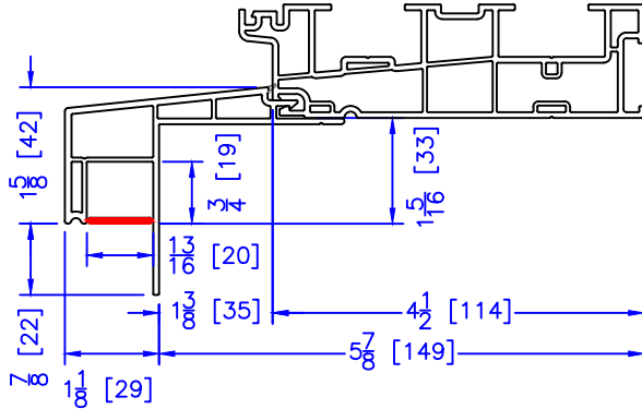
1-1/2" x 1-3/8" EXTENDED BM/J-TRIM
