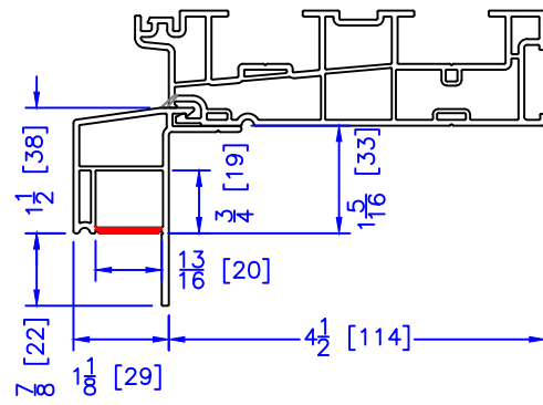
1-1/2" BM/J-TRIM
