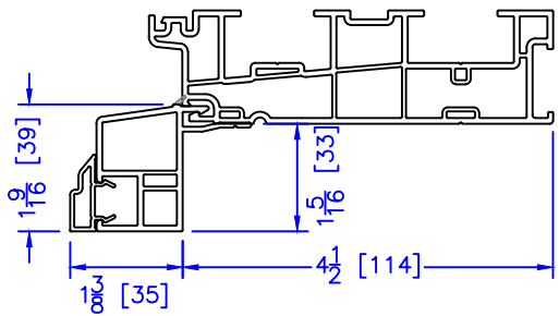
1-1/2" RENO BM
