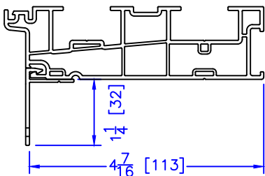
FLASHING FLANGE
