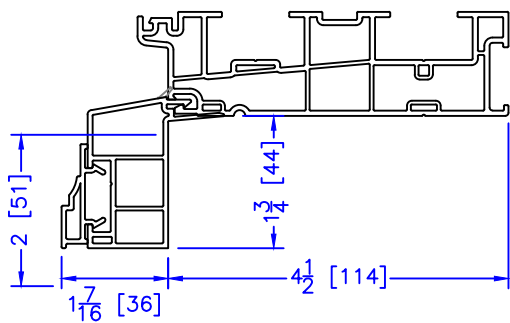
2" RENO BM
