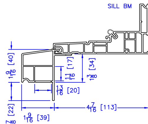
SILL BM
