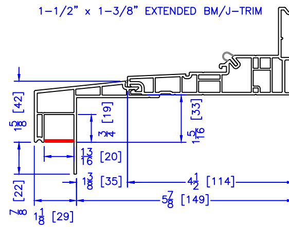
1-1/2" x 1-3/8" EXTENDED BM/J-TRIM
