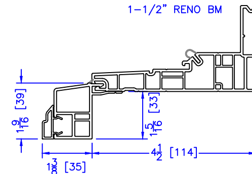
1-1/2" RENO BM
