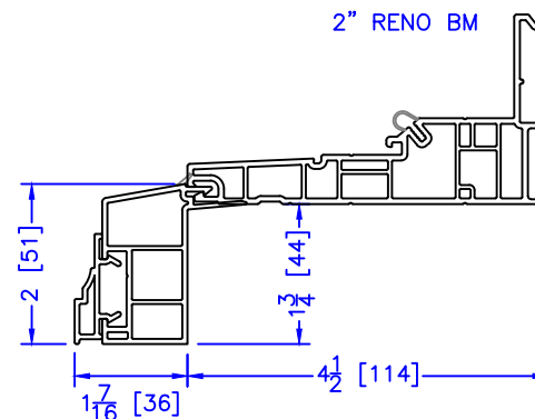
2" RENO BM
