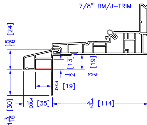
7/8" BM/J-TRIM
