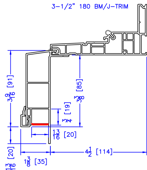
3-1/2" 180 BM/J-TRIM
