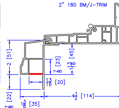
2" 180 BM/J-TRIM
