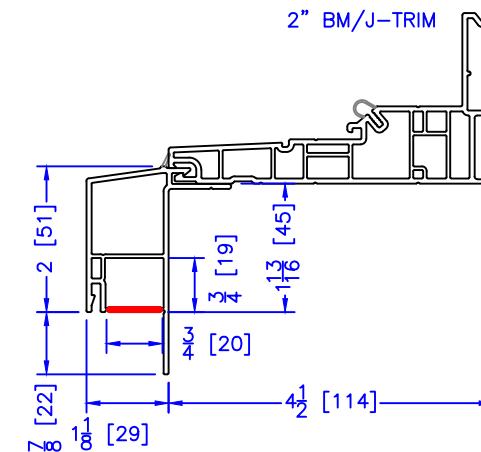
2" BM/J-TRIM
