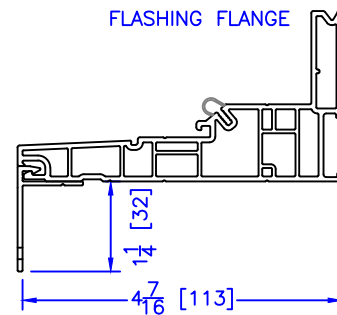
FLASHING FLANGE
