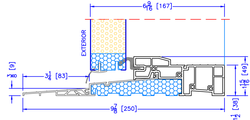
6 9/16" OUTSWING HIGH PERFORMANCE SILL 2 PC ALUMINUM (3 1/4" EXT) (SELECTABLE OPTION FOR ALL EXTERIOR OPTIONS)
