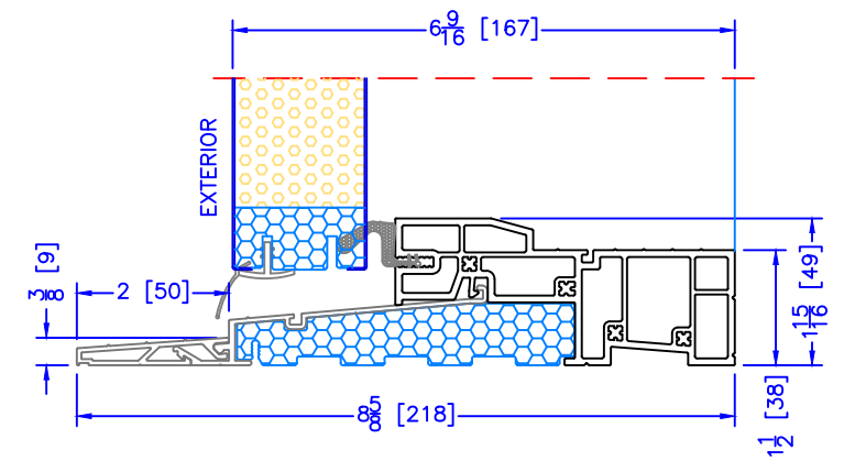
6 9/16" OUTSWING HIGH PERFORMANCE SILL 2 PC ALUMINUM (2" EXT) (SELECTABLE OPTION FOR ALL EXTERIOR OPTIONS)
