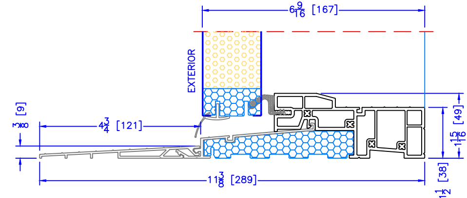
6 9/16" OUTSWING HIGH PERFORMANCE SILL 2 PC ALUMINUM (4 3/4" EXT) (SELECTABLE OPTION FOR ALL EXTERIOR OPTIONS)
