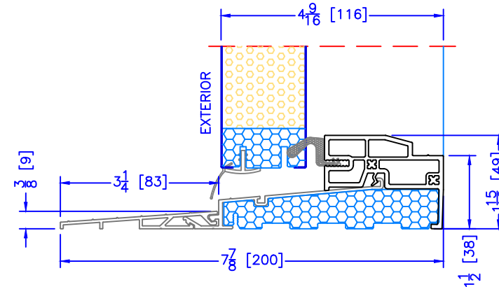
4 9/16" OUTSWING HIGH PERFORMANCE SILL 2 PC ALUMINUM (3 1/4" EXT) (SELECTABLE OPTION FOR ALL EXTERIOR OPTIONS)
