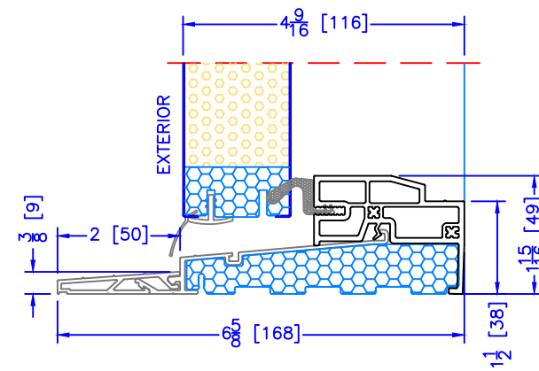
4 9/16" OUTSWING HIGH PERFORMANCE SILL 2 PC ALUMINUM (2" EXT) (SELECTABLE OPTION FOR ALL EXTERIOR OPTIONS)
