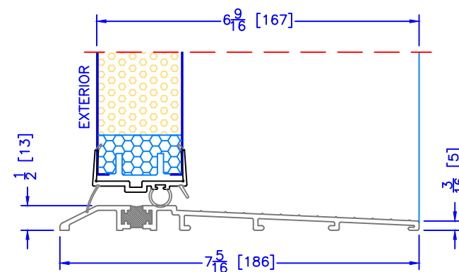
6 9/16" OUTSWING ASSISTED LIVING SILL
