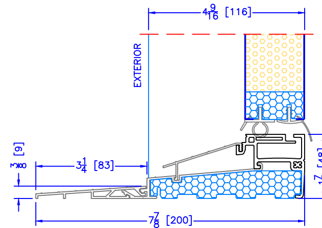
4 9/16" INSWING HIGH PERFORMANCE SILL 2 PC ALUMINUM (3 1/4" EXT) (SELECTABLE OPTION FOR ALL EXTERIOR OPTIONS)
