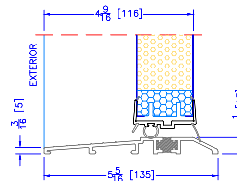
4 9/16" INSWING ASSISTED LIVING SILL
