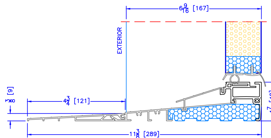
6 9/16" INSWING HIGH PERFORMANCE SILL 2 PC ALUMINUM (4 3/4" EXT) (SELECTABLE OPTION FOR ALL EXTERIOR OPTIONS)
