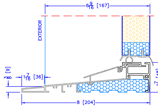
6 9/16" INSWING HIGH PERFORMANCE SILL 1 PC ALUMINUM (USED WITH 2" WOOD BM)
