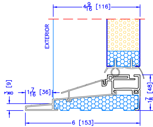
4 9/16" INSWING HIGH PERFORMANCE SILL 1 PC ALUMINUM (USED WITH 2" WOOD BM)
