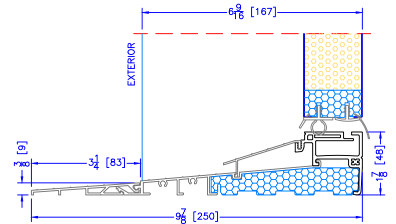
6 9/16" INSWING HIGH PERFORMANCE SILL 2 PC ALUMINUM (3 1/4" EXT) (SELECTABLE OPTION FOR ALL EXTERIOR OPTIONS)
