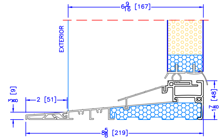
6 9/16" INSWING HIGH PERFORMANCE SILL 2 PC ALUMINUM (2" EXT) (USED WITH PLAIN FRAME)
