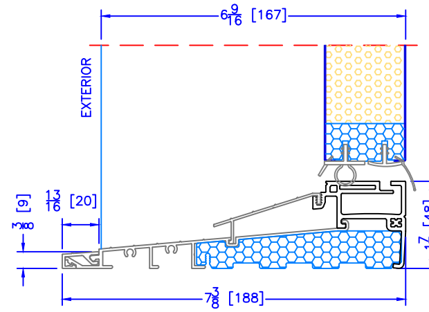
6 9/16" INSWING HIGH PERFORMANCE SILL CLOSE-OUT EXTENSION (USED WITH PLAIN FRAME)
