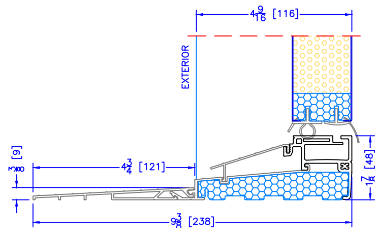
4 9/16" INSWING HIGH PERFORMANCE SILL 2 PC ALUMINUM (4 3/4" EXT) (SELECTABLE OPTION FOR ALL EXTERIOR OPTIONS)
