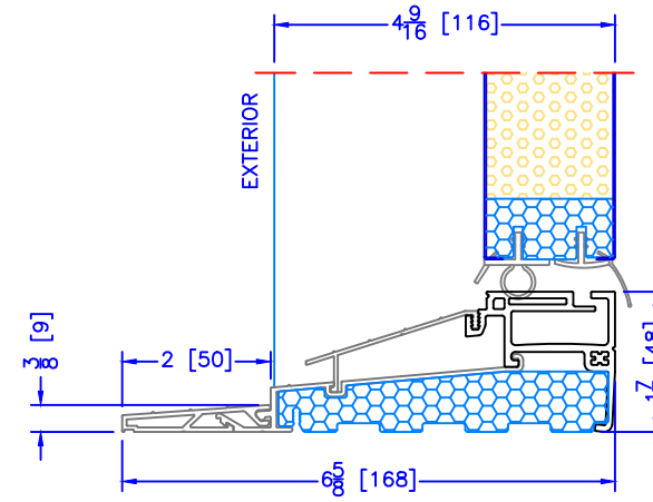
4 9/16" INSWING HIGH PERFORMANCE SILL 2 PC ALUMINUM (2" EXT) (USED WITH PLAIN FRAME)
