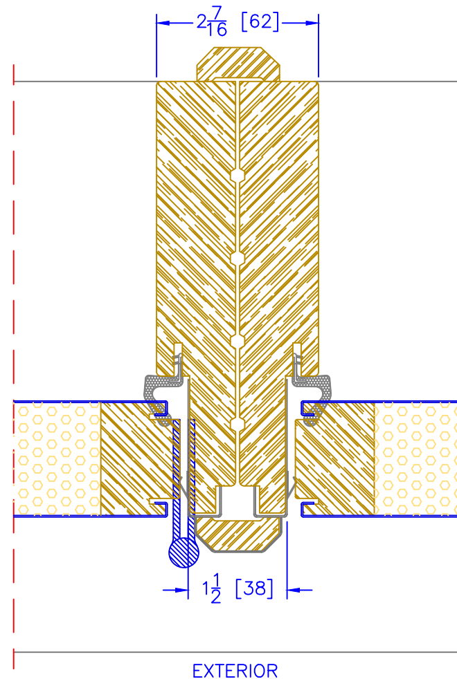
6 9 / 16 " OUTSWING OPERATOR/SIDELITE VERTICAL MULLION
