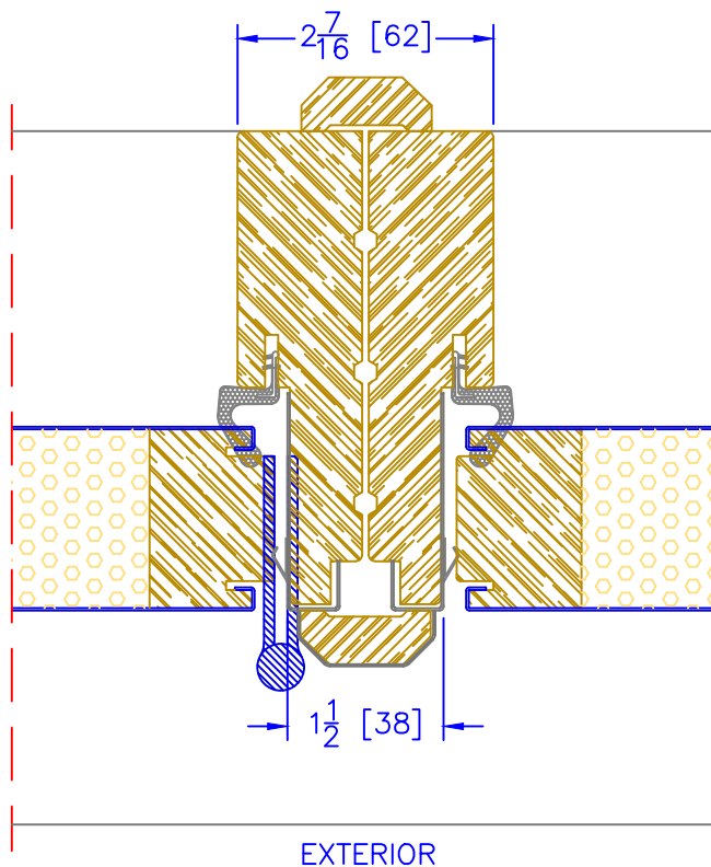
4 9 / 16 " OUTSWING OPERATOR/SIDELITE VERTICAL MULLION
