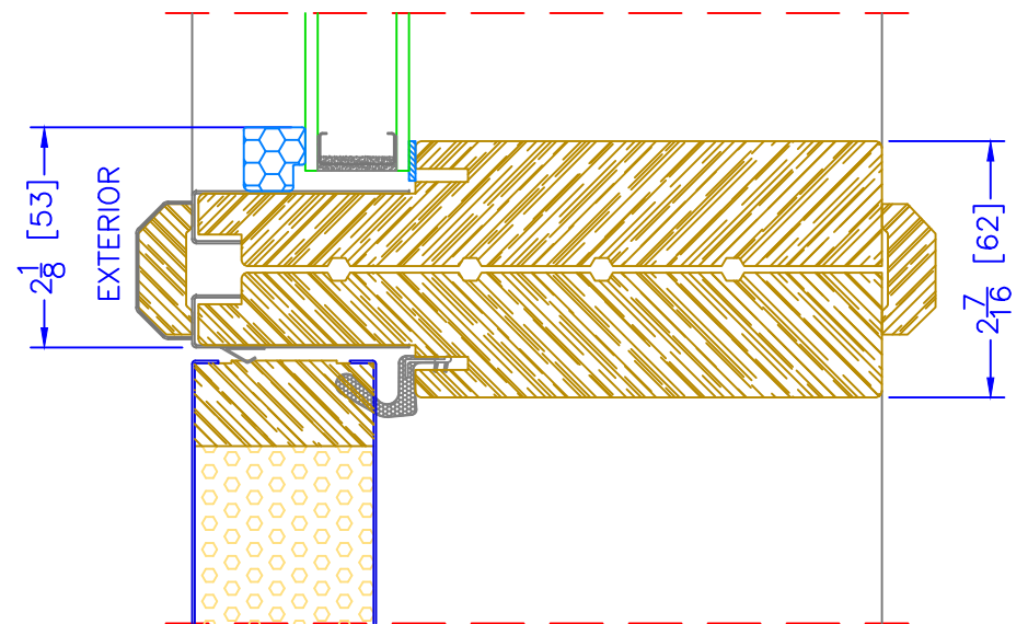
6 \frac{9}{16} " OUTSWING TRANSOM o/ OPERATOR HORIZONTAL MULLION
