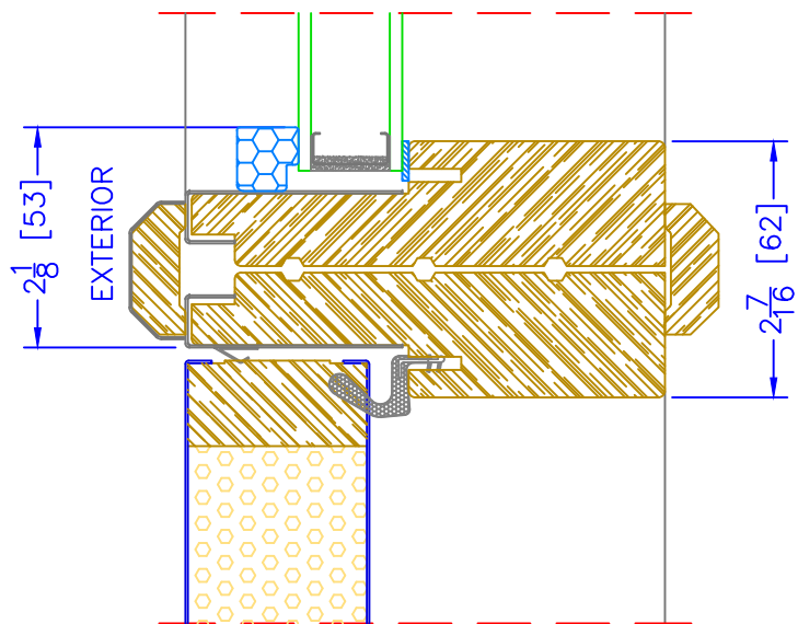
4 \frac{9}{16} " OUTSWING TRANSOM o/ OPERATOR HORIZONTAL MULLION
