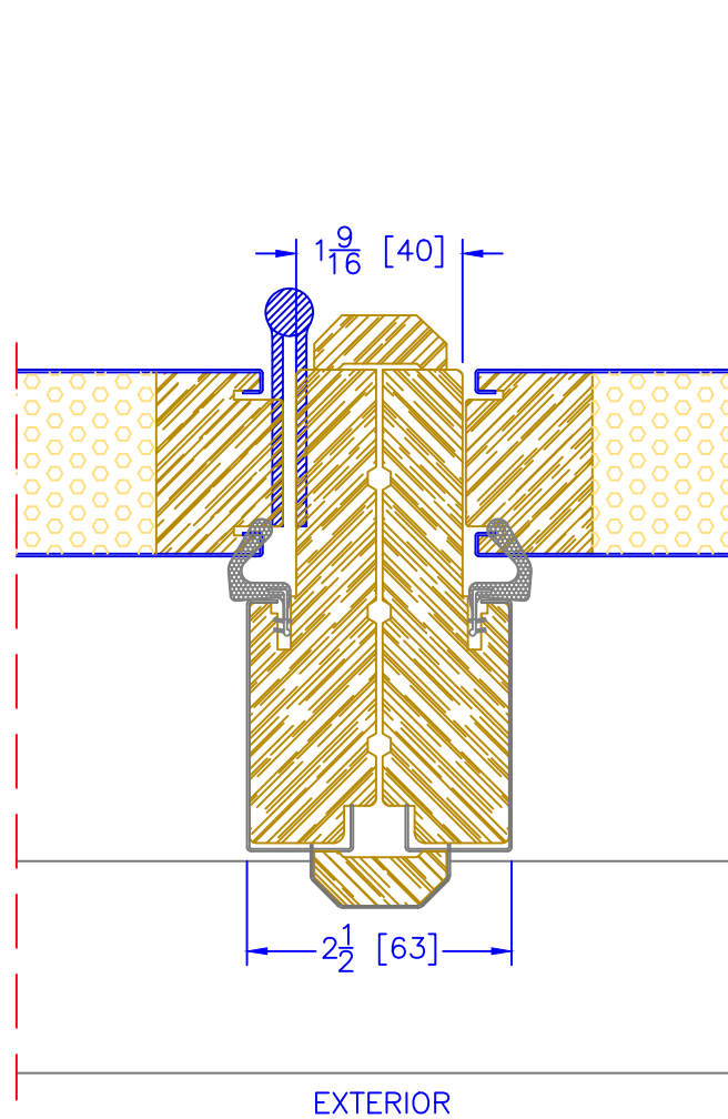
4 1/2" INSWING OPERATOR/SIDELITE VERTICAL MULLION
