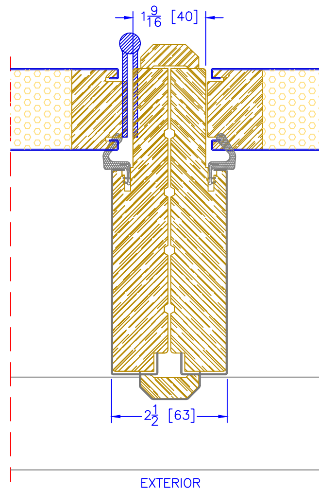
6 9/16" INSWING OPERATOR/SIDELITE VERTICAL MULLION
