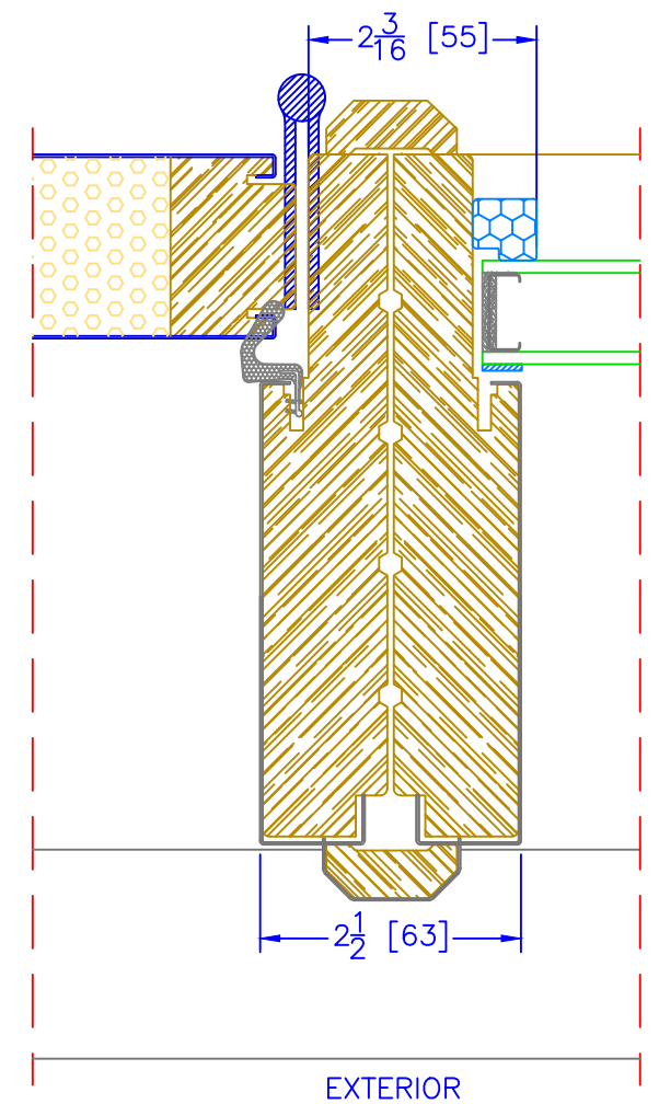
6 9/16" INSWING OPERATOR/S-100 VERTICAL MULLION
