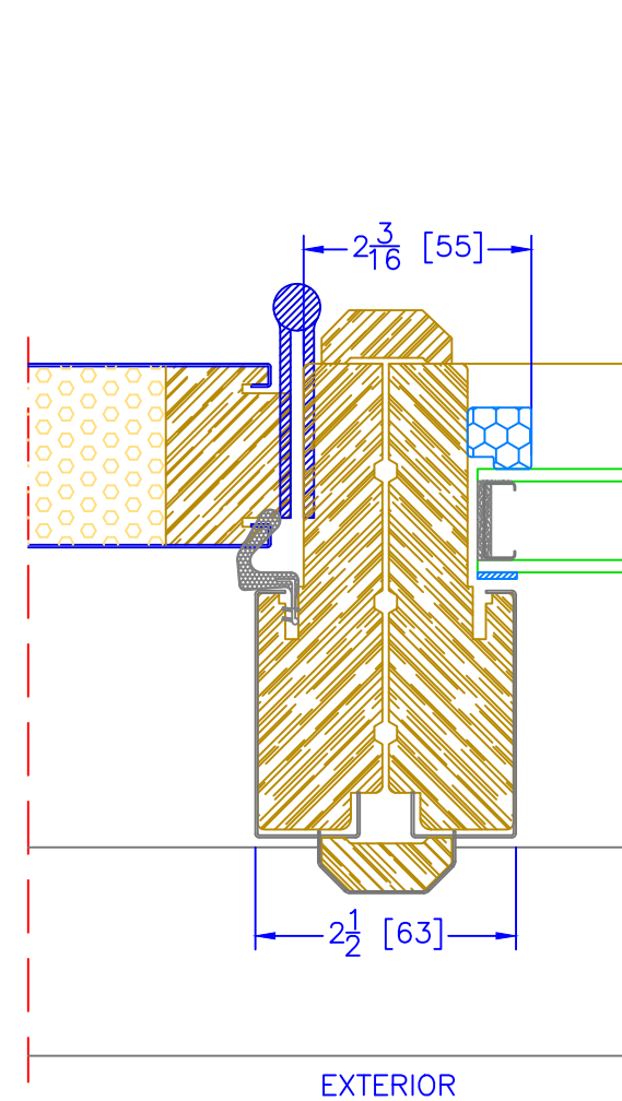
4 1/2" INSWING OPERATOR/S-100 VERTICAL MULLION
