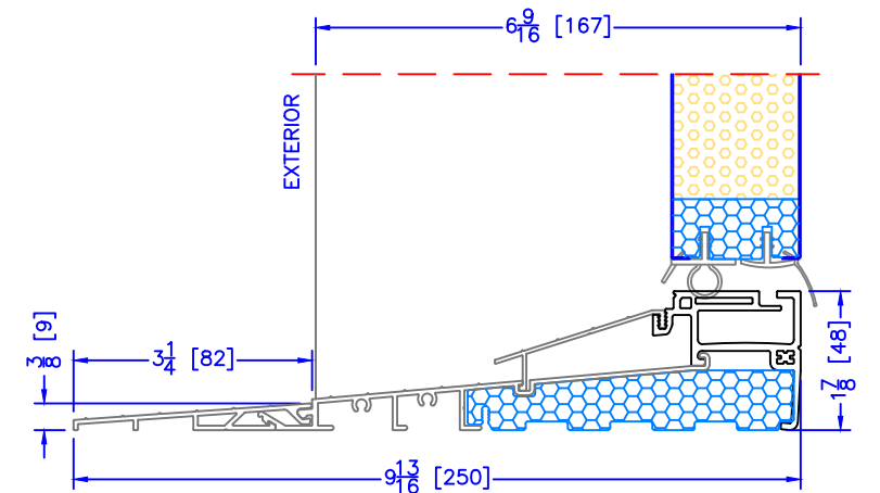
6 9/16" INSWING HIGH PERFORMANCE SILL 2 PC ALUMINUM (3-1/4" EXT) (SELECTABLE OPTION FOR ALL EXTERIOR OPTIONS)
