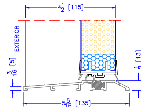
4 1/2" INSWING ASSISTED LIVING SILL
