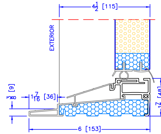
4 1/2" INSWING HIGH PERFORMANCE SILL 1 PC ALUMINUM (USED WITH 2" DOOR BM'S)
