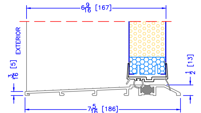
6 9/16" INSWING ASSISTED LIVING SILL
