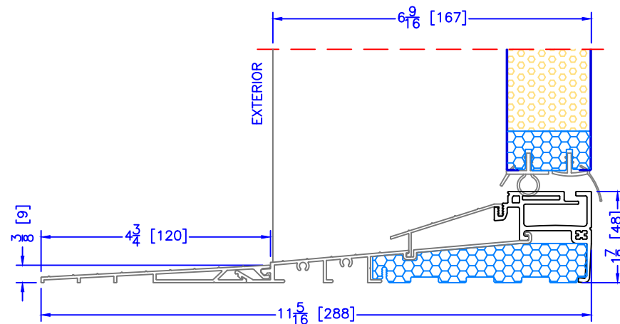
6 9/16" INSWING HIGH PERFORMANCE SILL 2 PC ALUMINUM (4-3/4" EXT) (SELECTABLE OPTION FOR ALL EXTERIOR OPTIONS)
