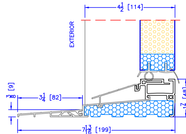
4 1/2" INSWING HIGH PERFORMANCE SILL 2 PC ALUMINUM (3-1/4" EXT) (SELECTABLE OPTION FOR ALL EXTERIOR OPTIONS)
