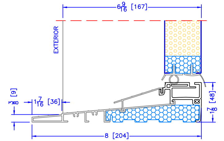
6 9/16" INSWING HIGH PERFORMANCE SILL 1 PC ALUMINUM (USED WITH 2" DOOR BM'S)
