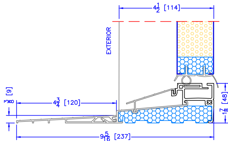
4 1/2" INSWING HIGH PERFORMANCE SILL 2 PC ALUMINUM (4-3/4" EXT) (SELECTABLE OPTION FOR ALL EXTERIOR OPTIONS)
