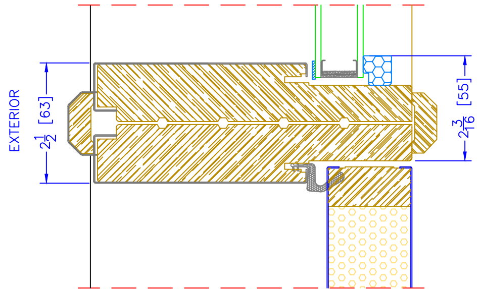
6 9/16" INSWING TRANSOM o/ OPERATOR HORIZONTAL MULLION
