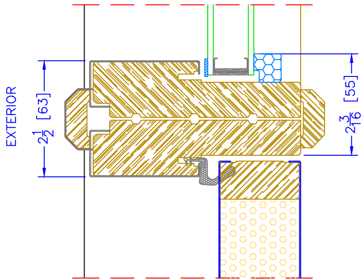
4 1/2" INSWING TRANSOM o/ OPERATOR HORIZONTAL MULLION
