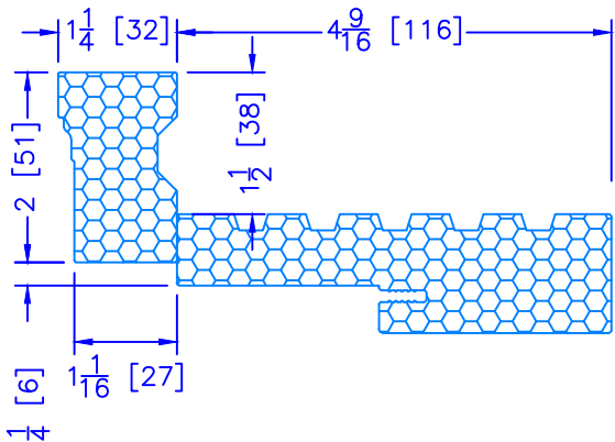
2" PVC DOOR BM (ONLY AVAILABLE w/ STAINABLE PVC FRAME)
