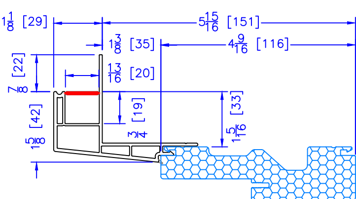
1-1/2" x 1-3/8" EXTENDED BM/J-TRIM
