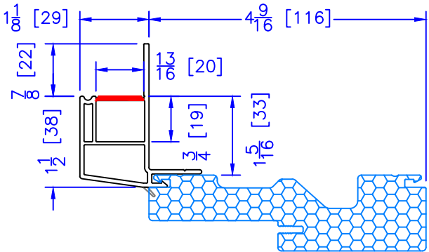
1-1/2" BM/J-TRIM
