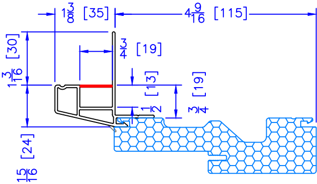
7/8" BM/J-TRIM
