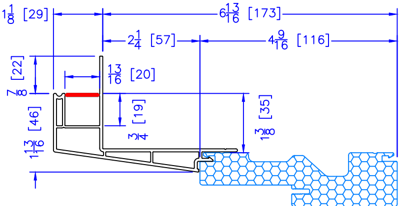
1-1/2" x 2-1/4" EXTENDED BM/J-TRIM (TO BE REVIEWED BY R&D)
