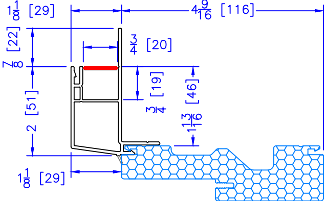
2" BM/J-TRIM
