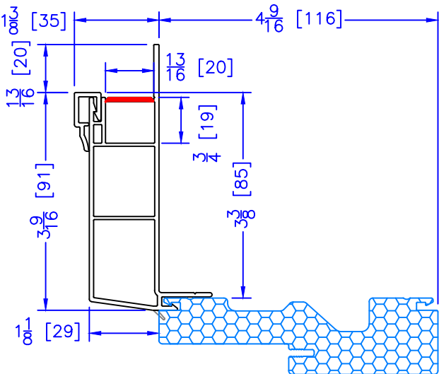
3-1/2" 180 BM/J-TRIM
