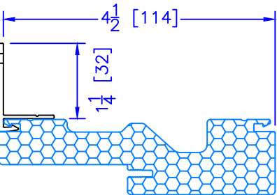
FLASHING FLANGE
