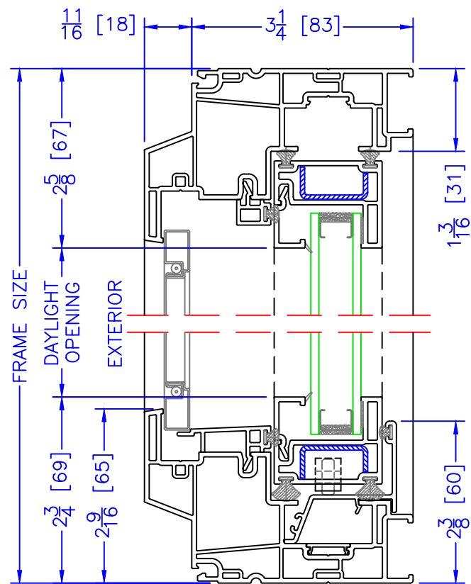
OPERATOR SASH HEAD/SILL
