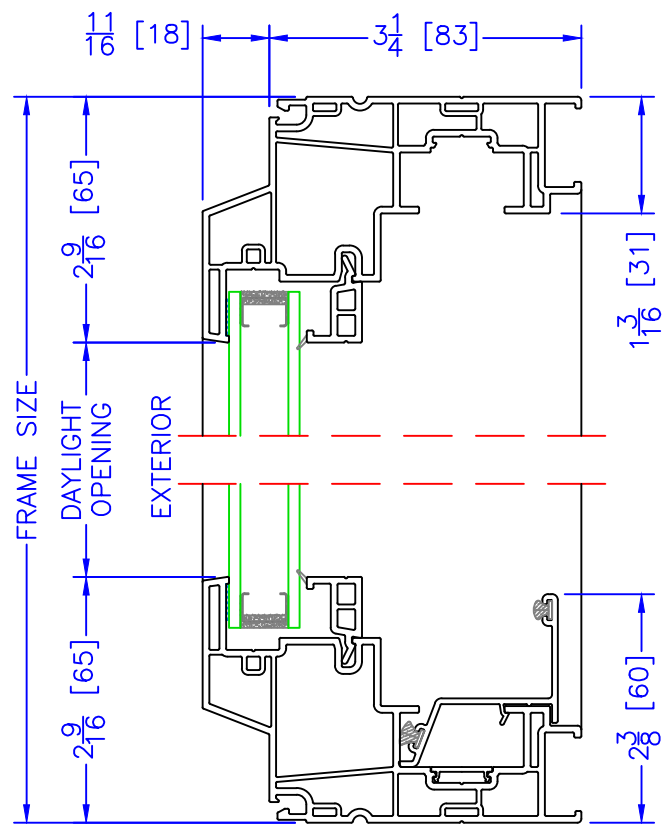
FIXED SASH HEAD/SILL
