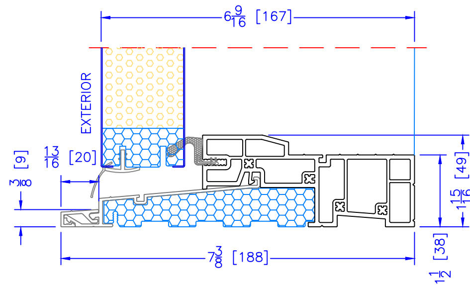
6 9 / 16 " OUTSWING HIGH PERFORMANCE SILL CLOSE-OUT EXTENSION (USED WITH PLAIN FRAME)
