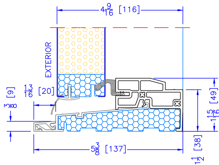
4 9 / 16 " OUTSWING HIGH PERFORMANCE SILL CLOSE-OUT EXTENSION (USED WITH PLAIN FRAME)
