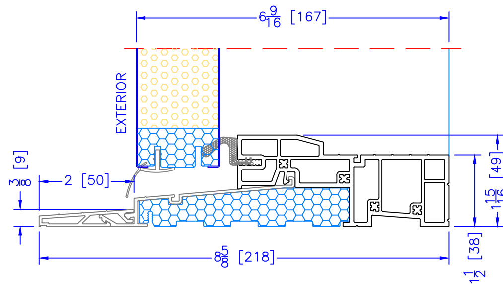
6 9 / 16 " OUTSWING HIGH PERFORMANCE SILL 2 PC ALUMINUM (2" EXT) (USED WITH 2" WOOD BM)
