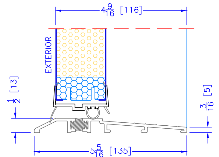
4 9 / 16 " OUTSWING ASSISTED LIVING SILL
