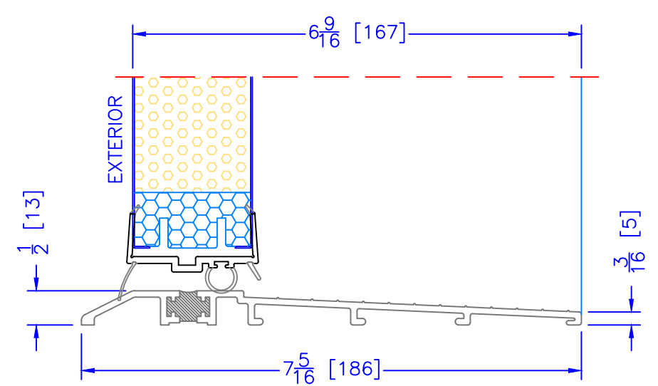
6 9 / 16 " OUTSWING ASSISTED LIVING SILL
