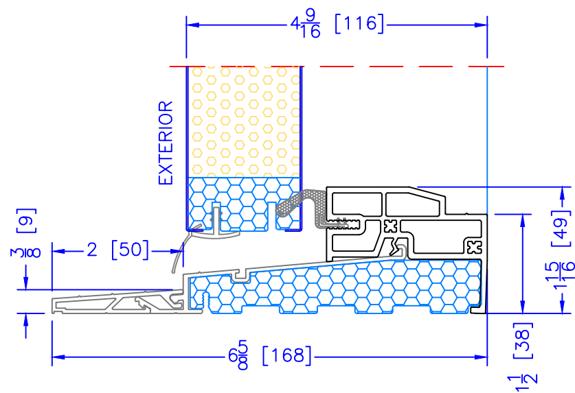
4 9 / 16 " OUTSWING HIGH PERFORMANCE SILL 2 PC ALUMINUM (2" EXT) (USED WITH 2" WOOD BM)
