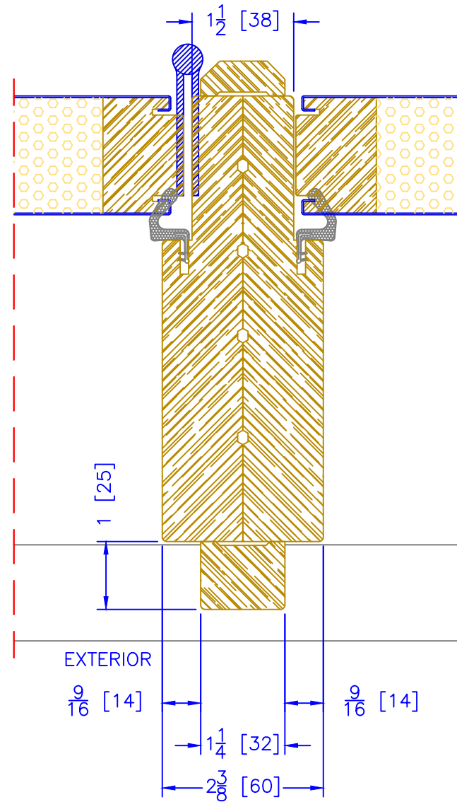
6 9 / 16 " INSWING OPERATOR/SIDELITE VERTICAL MULLION STORM DOOR PREP ON POST ONLY AVAILABLE w/ STORM DOOR PREP BRICKMOULDS
