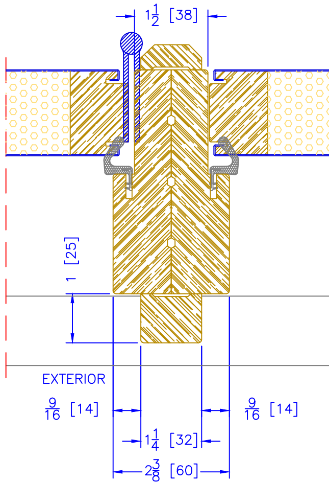
4 9 / 16 " INSWING OPERATOR/SIDELITE VERTICAL MULLION STORM DOOR PREP ON POST ONLY AVAILABLE w/ STORM DOOR PREP BRICKMOULDS
