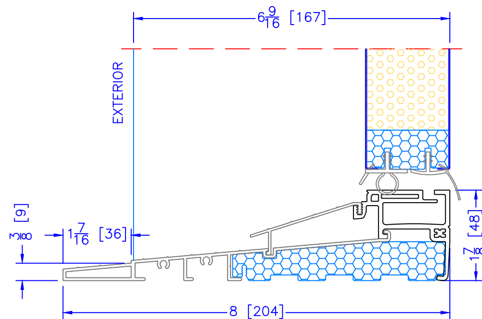
6 \frac{9}{16} " INSWING HIGH PERFORMANCE SILL 1" PC ALUMINUM (USED WITH 2" WOOD BM)
