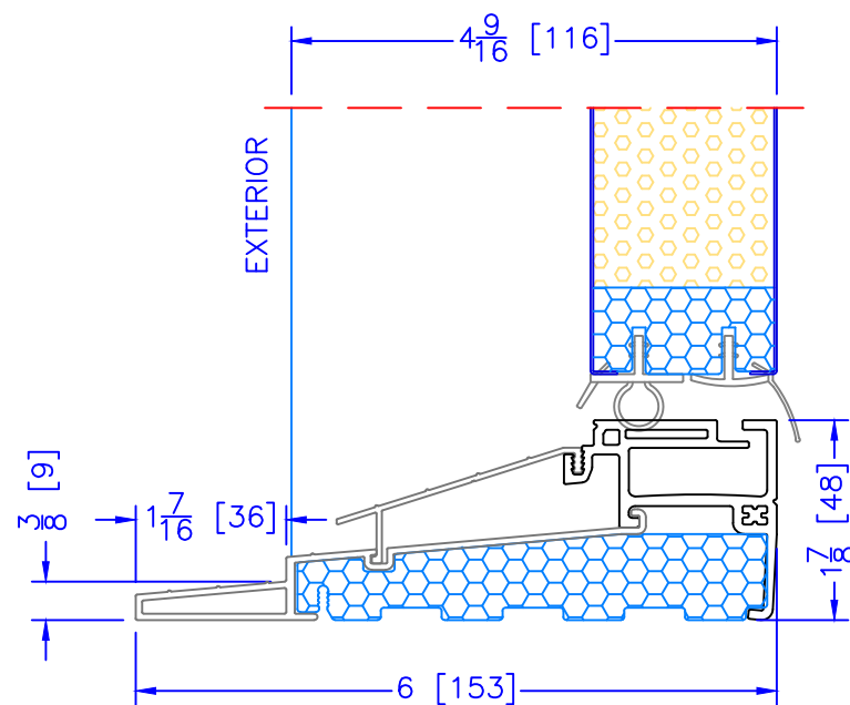
4 \frac{9}{16} " INSWING HIGH PERFORMANCE SILL 1" PC ALUMINUM (USED WITH 2" WOOD BM)
