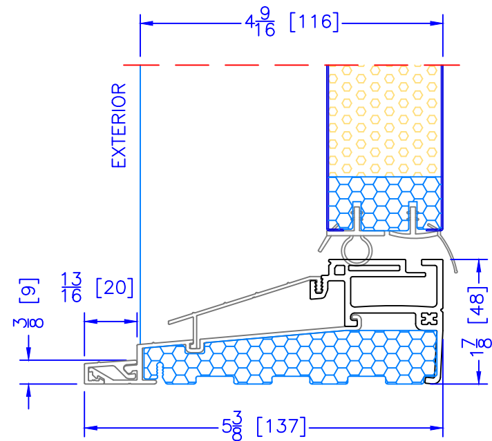
4 \frac{9}{16} " INSWING HIGH PERFORMANCE SILL CLOSE-OUT EXTENSION (USED WITH PLAIN FRAME)
