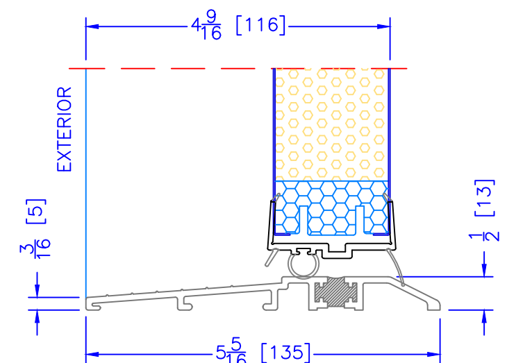
4 \frac{9}{16} " INSWING ASSISTED LIVING SILL
