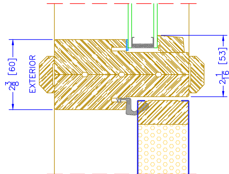
4 \frac{9}{16} " INSWING TRANSOM o/ OPERATOR HORIZONTAL MULLION
