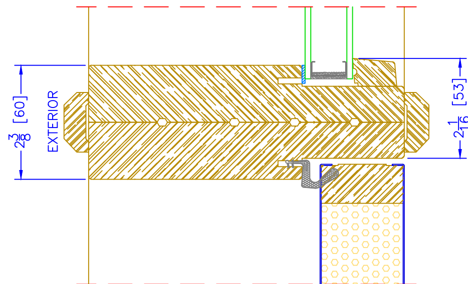
6 \frac{9}{16} " INSWING TRANSOM o/ OPERATOR HORIZONTAL MULLION
