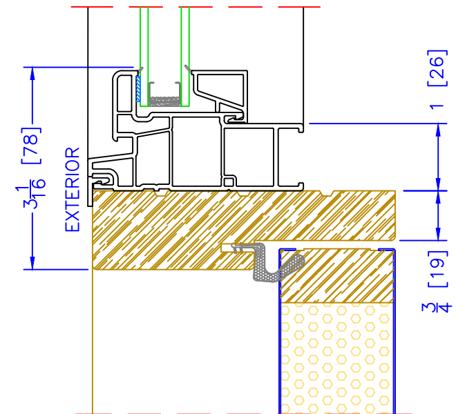
4 \frac{9}{16} " INSWING SHAPE o/ OPERATOR HORIZONTAL MULLION
