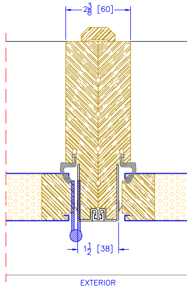
6 \frac{9}{16} " OUTSWING OPERATOR/SIDELITE VERTICAL MULLION
