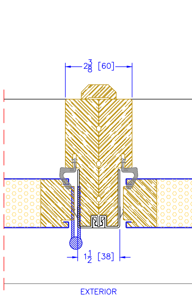
4 \frac{9}{16} " OUTSWING OPERATOR/SIDELITE VERTICAL MULLION
