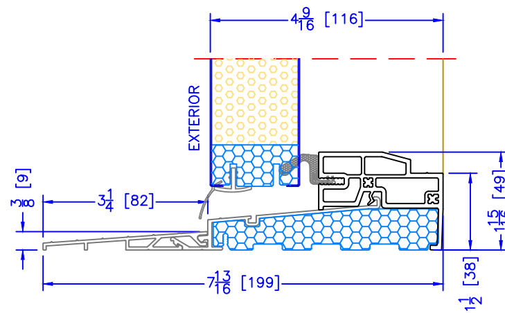
4 9/16" OUTSWING HIGH PERFORMANCE SILL 2 PC ALUMINUM (3 1/4" EXT) (USED WITH 1 1/2" EXTENDED BM/J-TRIM & FLUSH EXTENSION)
