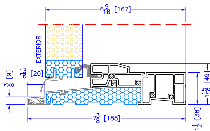
6 9/16" OUTSWING HIGH PERFORMANCE SILL CLOSE-OUT EXTENSION (USED WITH PLAIN FRAME)
