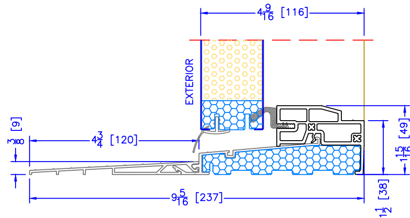
4 9/16" OUTSWING HIGH PERFORMANCE SILL 2 PC ALUMINUM (4 3/4" EXT) (USED WITH 1 1/2" EXTENDED BM/J-TRIM)
