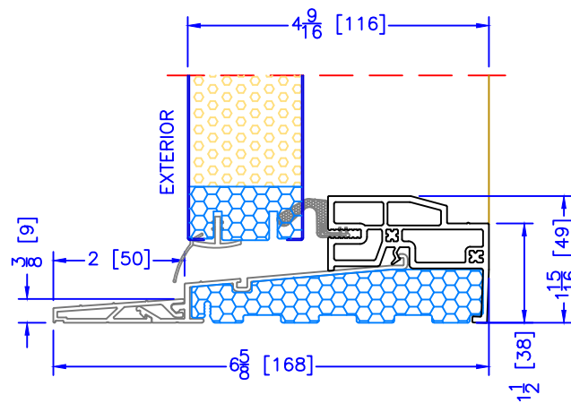
4 9/16" OUTSWING HIGH PERFORMANCE SILL 2 PC ALUMINUM (2" EXT) (USED WITH ALL OTHER EXTERIOR OPTIONS)
