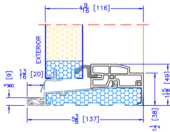
4 9/16" OUTSWING HIGH PERFORMANCE SILL CLOSE-OUT EXTENSION (USED WITH PLAIN FRAME)
