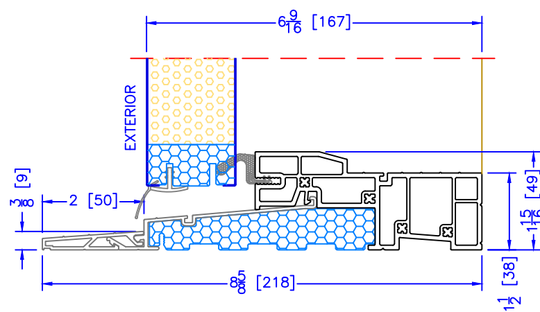
6 9/16" OUTSWING HIGH PERFORMANCE SILL 2 PC ALUMINUM (2" EXT) (USED WITH ALL OTHER EXTERIOR OPTIONS)
