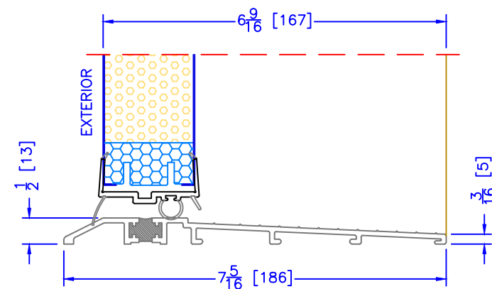
6 9/16" OUTSWING ASSISTED LIVING SILL
