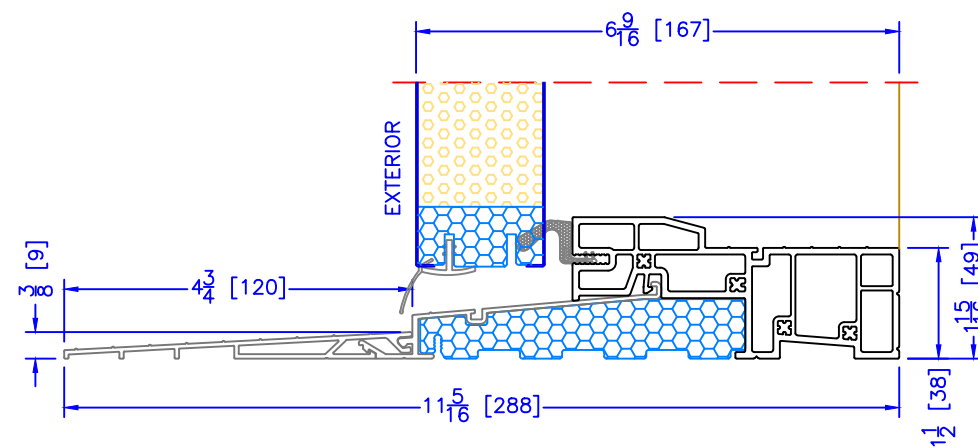
6 9/16" OUTSWING HIGH PERFORMANCE SILL 2 PC ALUMINUM (4 3/4" EXT) (USED WITH 1 1/2" EXTENDED BM/J-TRIM)
