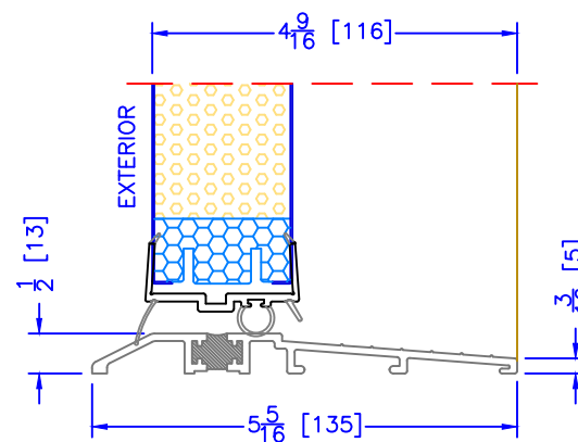
4 9/16" OUTSWING ASSISTED LIVING SILL
