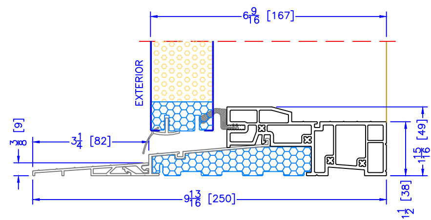
6 9/16" OUTSWING HIGH PERFORMANCE SILL 2 PC ALUMINUM (3 1/4" EXT) (USED WITH 1 1/2" EXTENDED BM/J-TRIM & FLUSH EXTENSION)
