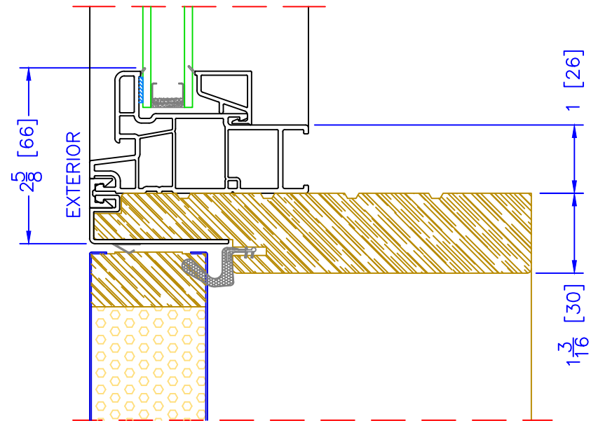
6 9 / 16 " OUTSWING SHAPE o/ OPERATOR HORIZONTAL MULLION
