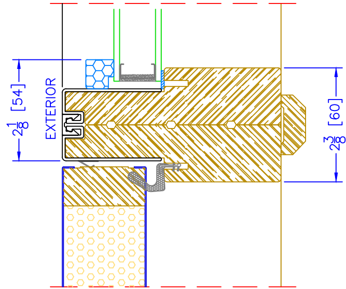
4 9 / 16 " OUTSWING TRANSOM o/ OPERATOR HORIZONTAL MULLION
