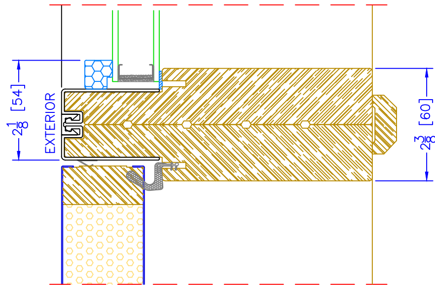
6 9 / 16 " OUTSWING TRANSOM o/ OPERATOR HORIZONTAL MULLION
