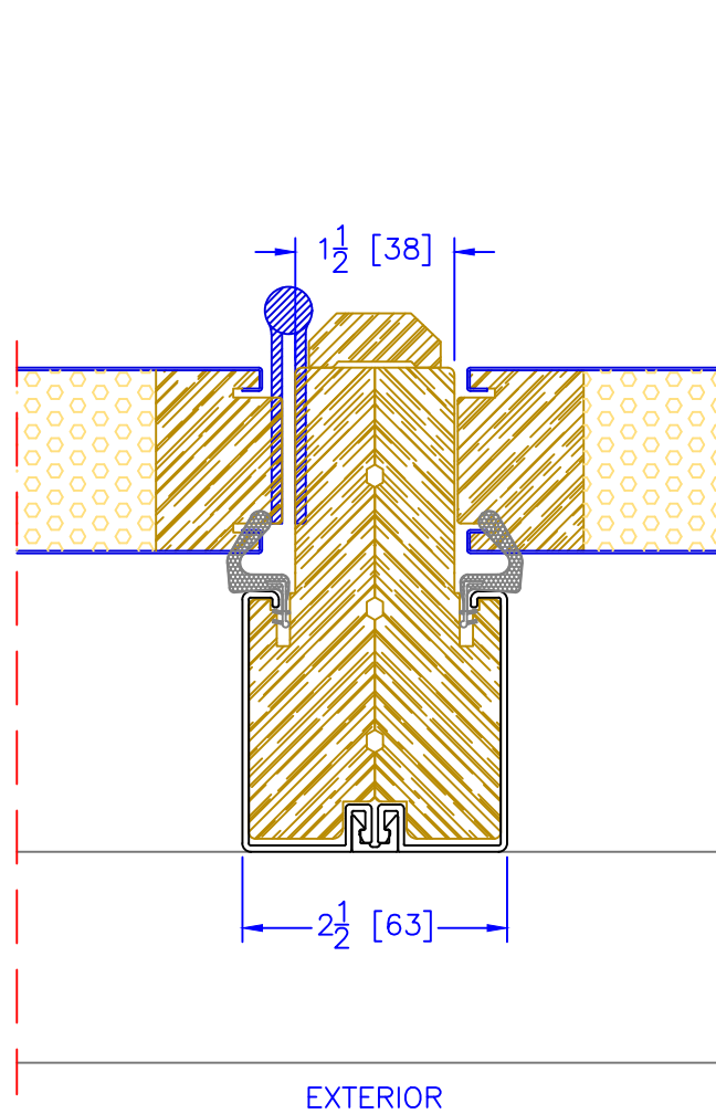
4 9 / 16 " INSWING OPERATOR/SIDELITE VERTICAL MULLION
