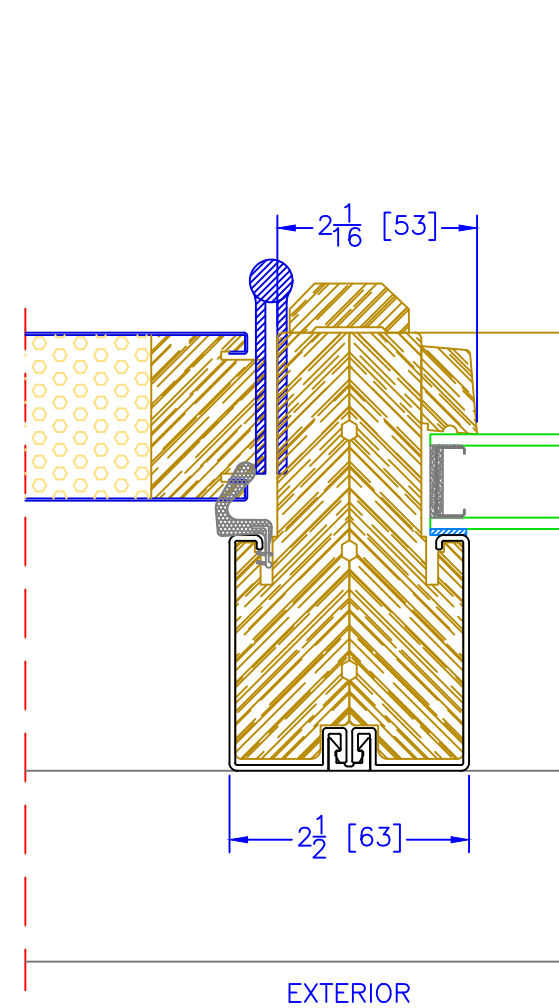
4 9 / 16 " INSWING OPERATOR/S-100 VERTICAL MULLION
