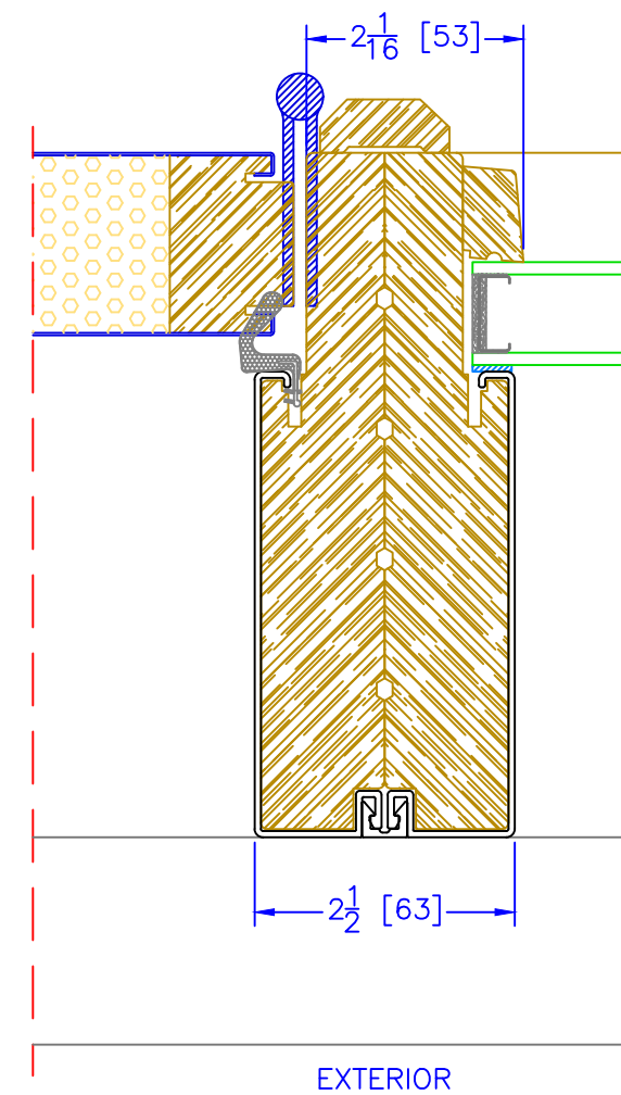
6 9 / 16 " INSWING OPERATOR/S-100 VERTICAL MULLION
