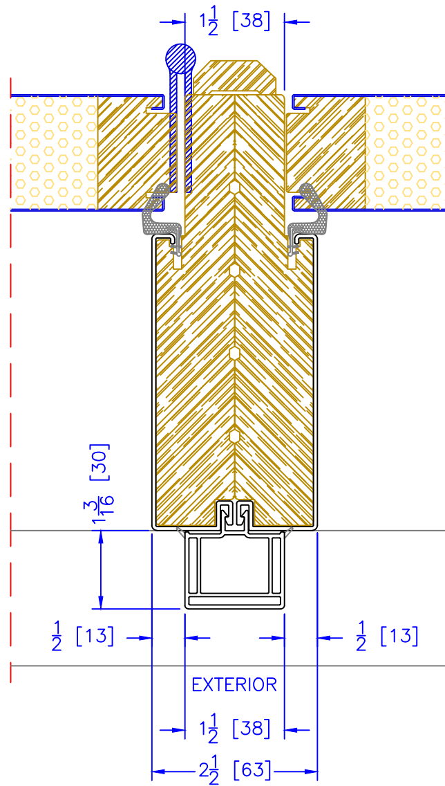
6 \frac{9}{16} " INSWING OPERATOR/SIDELITE VERTICAL MULLION STORM DOOR PREP ON POST ONLY AVAILABLE w/ STORM DOOR PREP BRICKMOULDS
