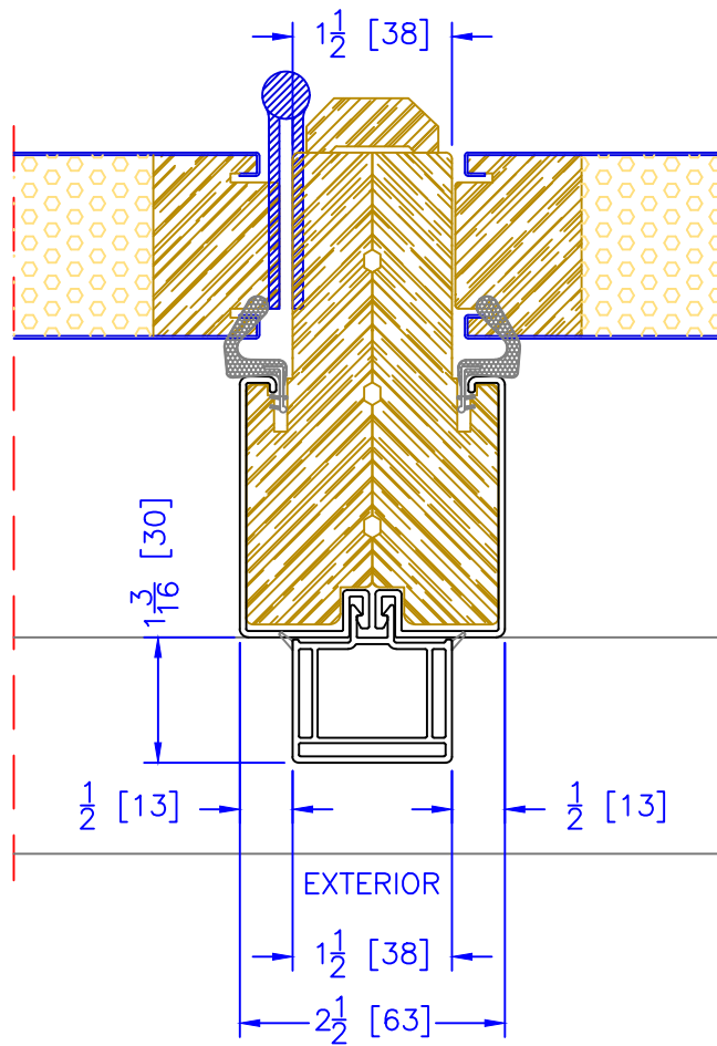
4 \frac{9}{16} " INSWING OPERATOR/SIDELITE VERTICAL MULLION STORM DOOR PREP ON POST ONLY AVAILABLE w/ STORM DOOR PREP BRICKMOULDS
