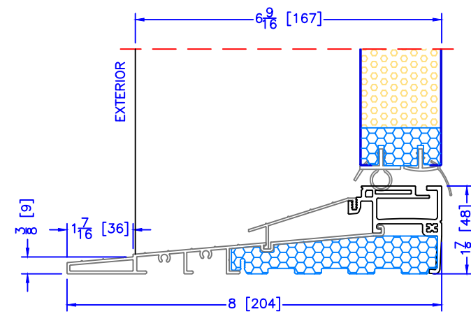
6-9/16" INSWING HIGH PERFORMANCE SILL 1 PC ALUMINUM (USED WITH 2" DOOR BM'S/J-TRIM'S)
