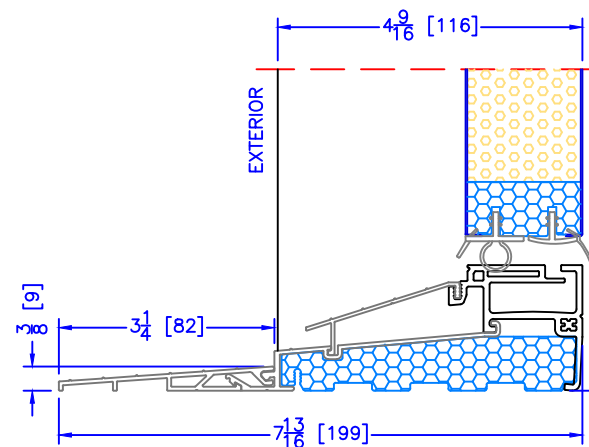
4-9/16" INSWING HIGH PERFORMANCE SILL 2 PC ALUMINUM (3/4" EXT) (USED WITH FLUSH EXTENSION)
