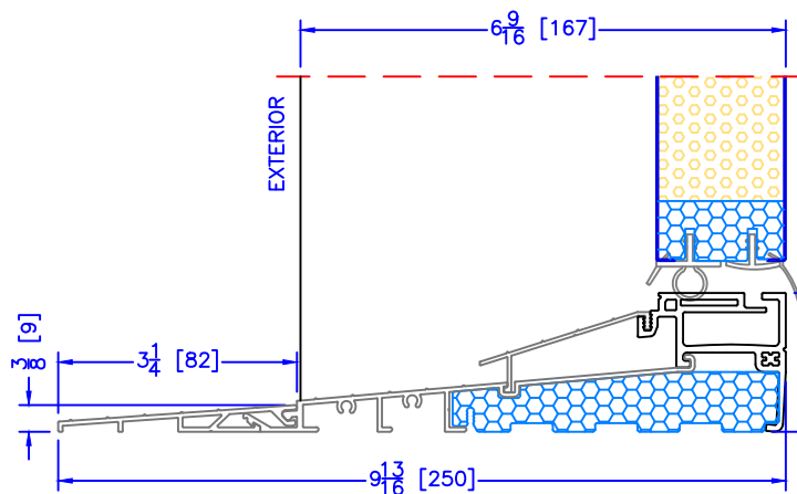
6-9/16" INSWING HIGH PERFORMANCE SILL 2 PC ALUMINUM (3/4" EXT) (USED WITH FLUSH EXTENSION)
