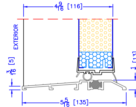
4-9/16" INSWING ASSISTED LIVING SILL
