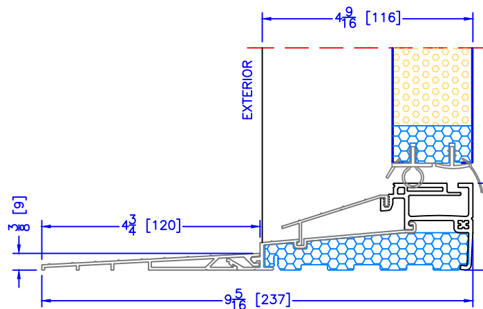
4-9/16" INSWING HIGH PERFORMANCE SILL 2 PC ALUMINUM (4 3/4" EXT) (USED WITH 1 1/2" EXTENDED BM/J-TRIM)
