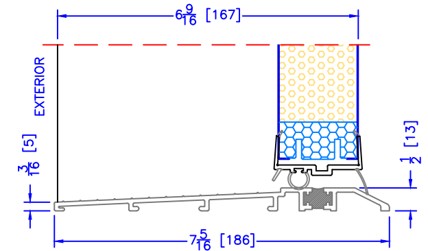
6-9/16" INSWING ASSISTED LIVING SILL
