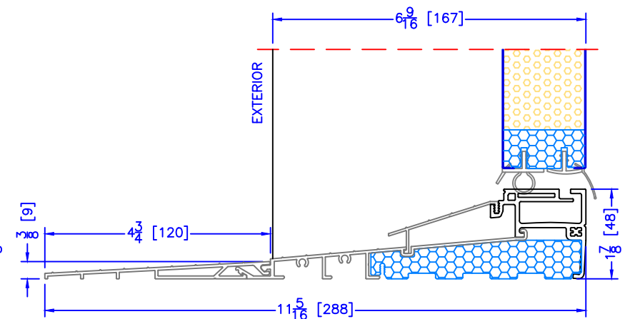
6-9/16" INSWING HIGH PERFORMANCE SILL 2 PC ALUMINUM (4 3/4" EXT) (USED WITH 1 1/2" EXTENDED BM/J-TRIM)
