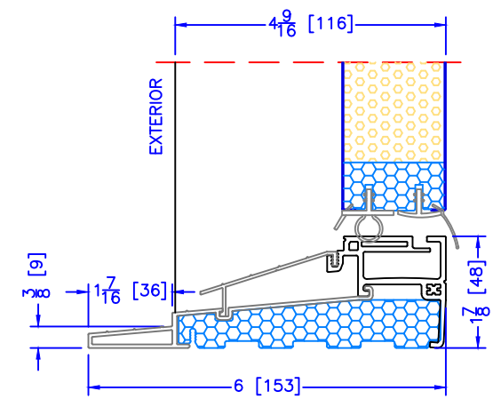
4-9/16" INSWING HIGH PERFORMANCE SILL 1 PC ALUMINUM (USED WITH 2" DOOR BM'S/J-TRIM'S)
