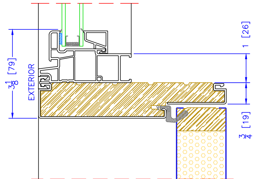
6 9 / 16 " INSWING SHAPE o/ OPERATOR HORIZONTAL MULLION
