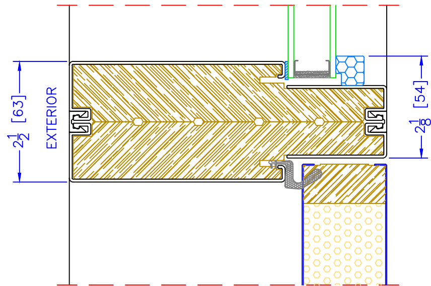
6 9 / 16 " INSWING TRANSOM o/ OPERATOR HORIZONTAL MULLION
