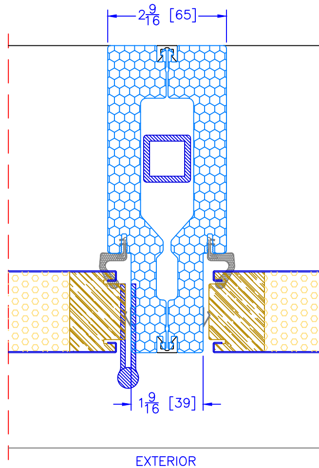
6 \frac{9}{16} " OUTSWING OPERATOR/SIDELITE VERTICAL MULLION
