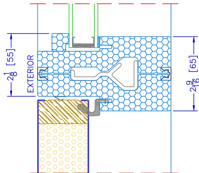
4 9 / 16 " OUTSWING TRANSOM/SHAPE o/ OPERATOR HORIZONTAL MULLION
