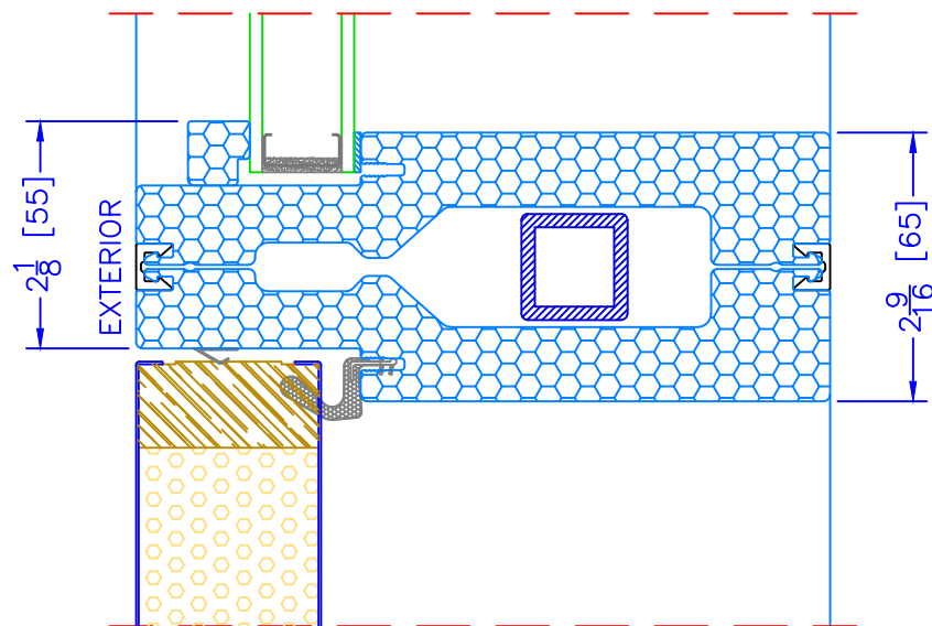
6 9 / 16 " OUTSWING TRANSOM/SHAPE o/ OPERATOR HORIZONTAL MULLION
