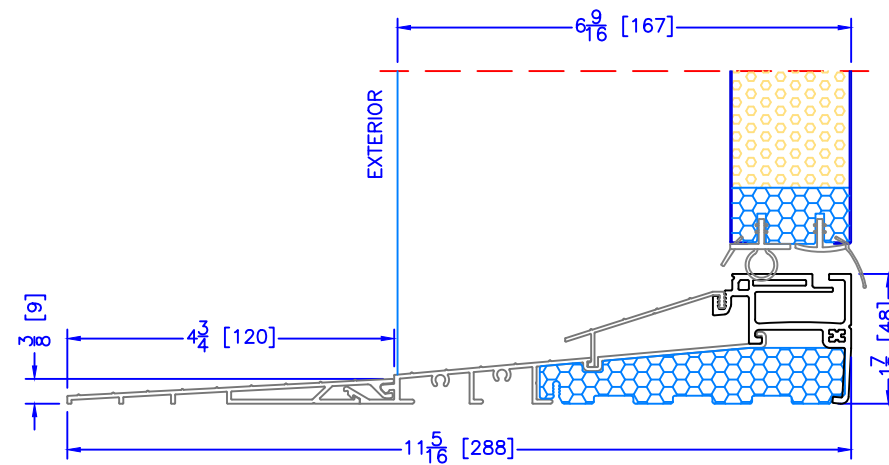
6 9/16" INSWING HIGH PERFORMANCE SILL 2 PC ALUMINUM (4 3/4" EXT) (USED WITH 1 1/2" EXTENDED BM/J-TRIM)
