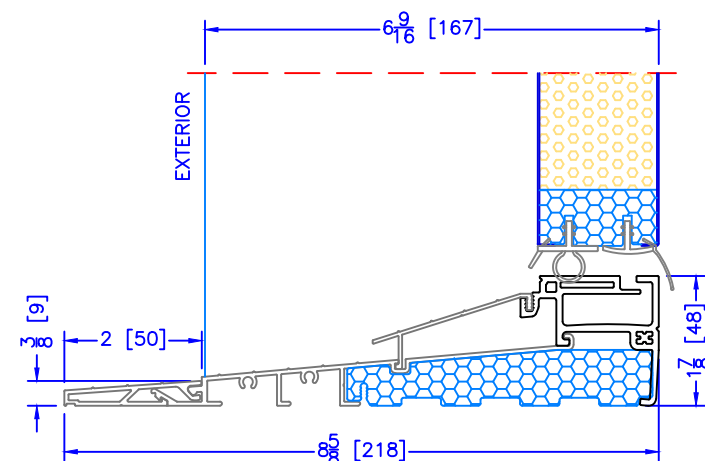
6 9/16" INSWING HIGH PERFORMANCE SILL 2 PC ALUMINUM (2" EXT) (USED WITH ALL OTHER EXTERIOR OPTIONS)
