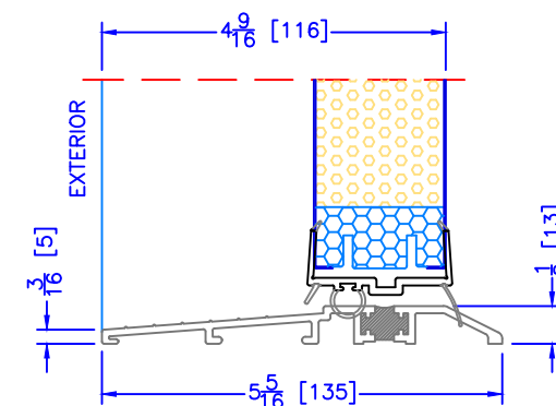
4 9/16" INSWING ASSISTED LIVING SILL
