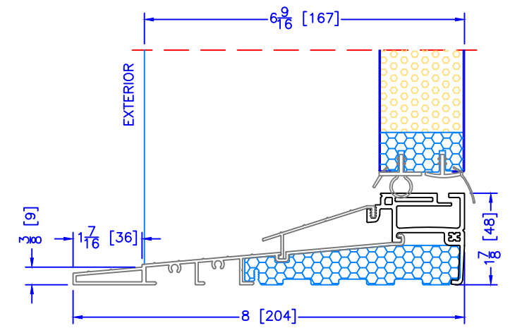
6 9/16" INSWING HIGH PERFORMANCE SILL 1 PC ALUMINUM (USED WITH 2" DOOR BM'S/J-TRIM'S)
