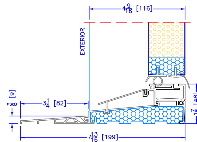
4 9/16" INSWING HIGH PERFORMANCE SILL 2 PC ALUMINUM (3/4" EXT) (USED WITH FLUSH EXTENSION)
