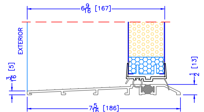
6 9/16" INSWING ASSISTED LIVING SILL
