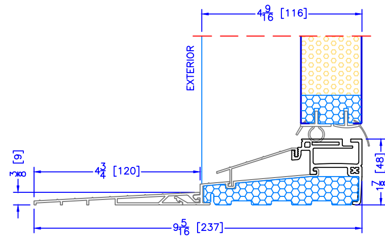
4 9/16" INSWING HIGH PERFORMANCE SILL 2 PC ALUMINUM (4 3/4" EXT) (USED WITH 1 1/2" EXTENDED BM/J-TRIM)
