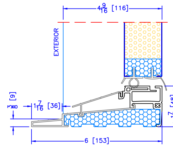
4 9/16" INSWING HIGH PERFORMANCE SILL 1 PC ALUMINUM (USED WITH 2" DOOR BM'S/J-TRIM'S)
