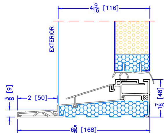
4 9/16" INSWING HIGH PERFORMANCE SILL 2 PC ALUMINUM (2" EXT) (USED WITH ALL OTHER EXTERIOR OPTIONS)
