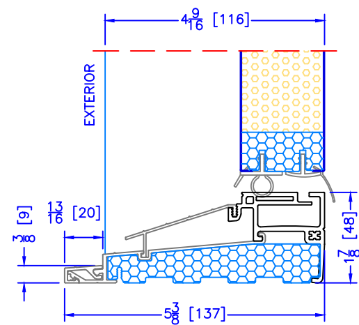
4 9/16" INSWING HIGH PERFORMANCE SILL CLOSE-OUT EXTENSION (USED WITH PLAIN FRAME)
