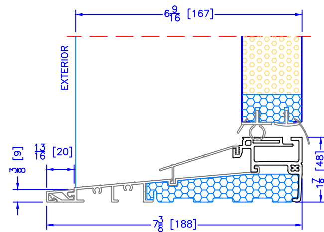
6 9/16" INSWING HIGH PERFORMANCE SILL CLOSE-OUT EXTENSION (USED WITH PLAIN FRAME)
