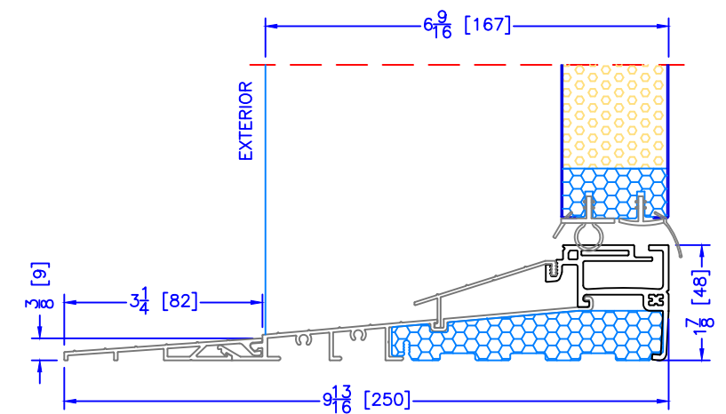
6 9/16" INSWING HIGH PERFORMANCE SILL 2 PC ALUMINUM (3/4" EXT) (USED WITH FLUSH EXTENSION)
