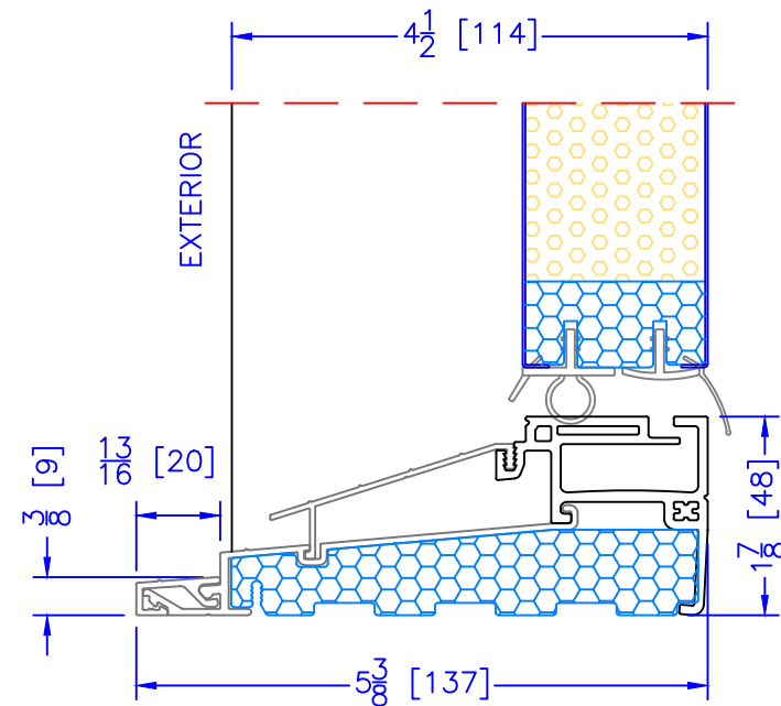
4 1/2" INSWING HIGH PERFORMANCE SILL CLOSE-OUT EXTENSION (USED WITH PLAIN FRAME)
