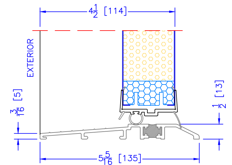
4 1/2" INSWING ASSISTED LIVING SILL
