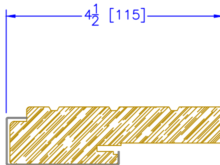
2" WOOD DOOR BM (AVAILABLE w/ STORM DOOR PREP) (N/A w/ SHAPES)
