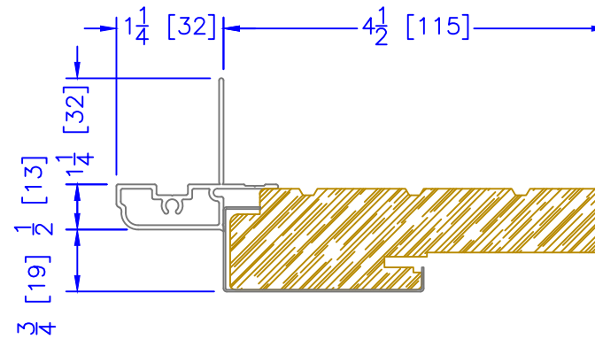
SLIM LINE BM
