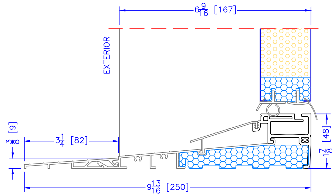
6 \frac{9}{16} " INSWING HIGH PERFORMANCE SILL 2 PC ALUMINUM (3 \frac{1}{4} " EXT) (USED WITH 1 \frac{1}{2} " EXTENDED BM/J-TRIM & FLUSH EXTENSION)
