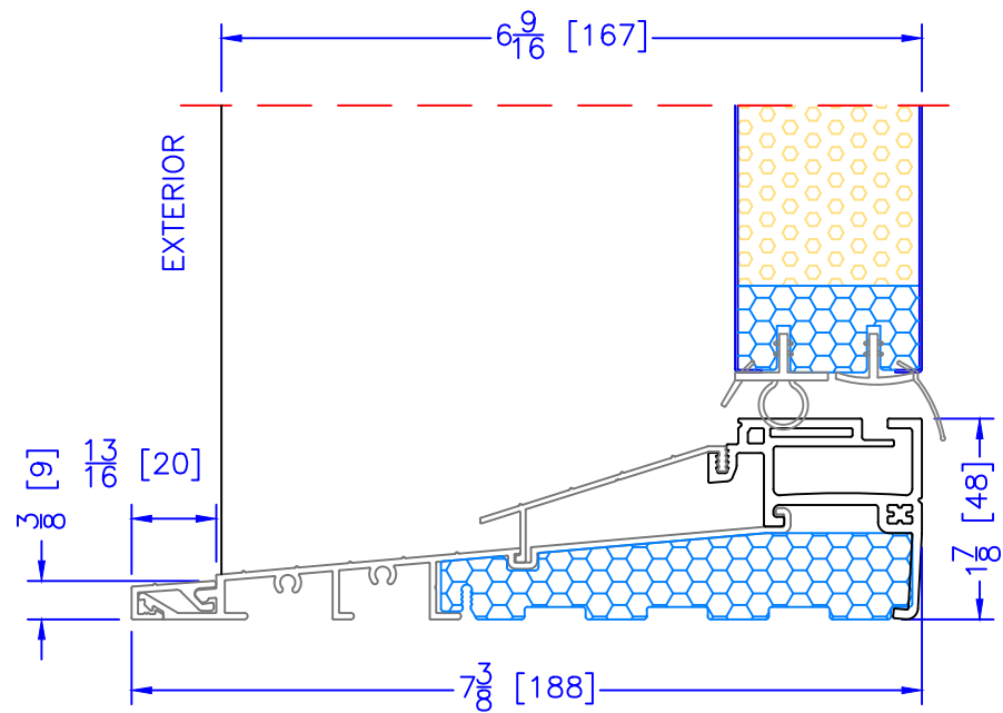
6 \frac{9}{16} " INSWING HIGH PERFORMANCE SILL CLOSE-OUT EXTENSION (USED WITH PLAIN FRAME)
