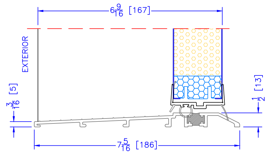
6 \frac{9}{16} " INSWING ASSISTED LIVING SILL
