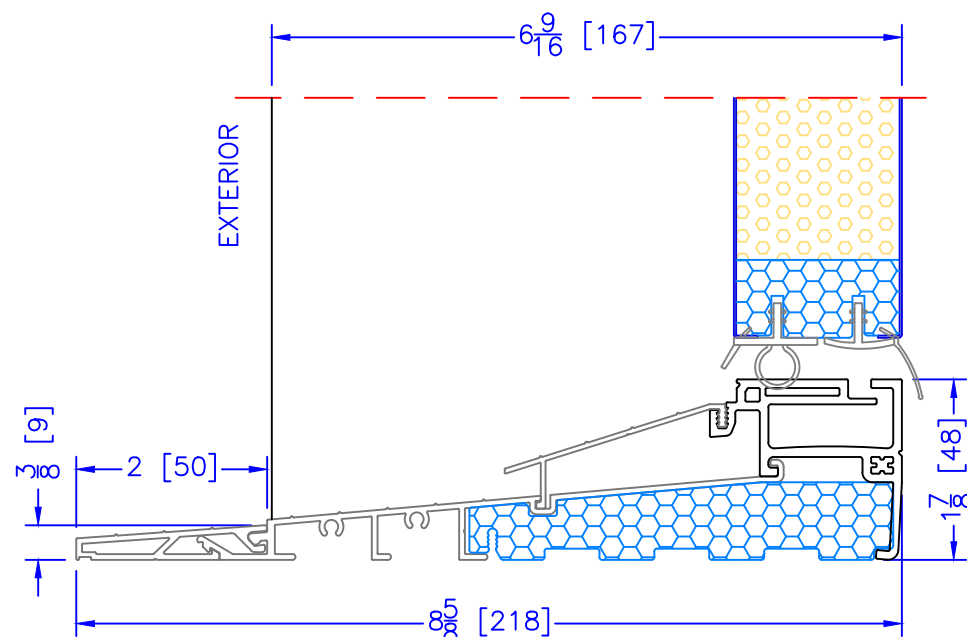
6 \frac{9}{16} " INSWING HIGH PERFORMANCE SILL 2 PC ALUMINUM (2" EXT) (USED WITH ALL OTHER EXTERIOR OPTIONS)
