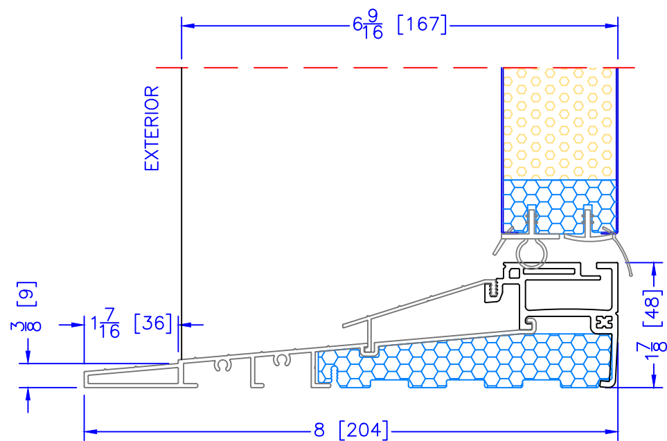
6 \frac{9}{16} " INSWING HIGH PERFORMANCE SILL 1 PC ALUMINUM (USED WITH 2" DOOR BM'S/J-TRIM'S)
