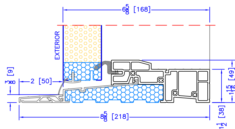
6 5/8" OUTSWING HIGH PERFORMANCE SILL 2 PC ALUMINUM (2" EXT) (USED WITH ALL OTHER EXTERIOR OPTIONS)
