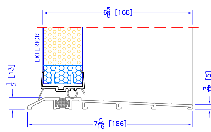
6 5/8" OUTSWING ASSISTED LIVING SILL
