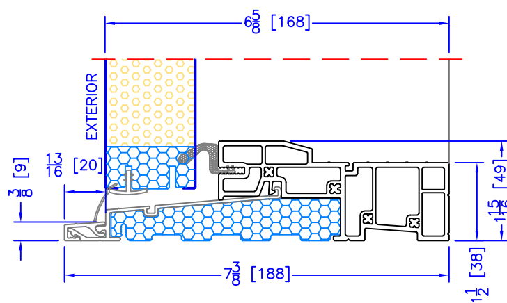
6 5/8" OUTSWING HIGH PERFORMANCE SILL CLOSE-OUT EXTENSION (USED WITH PLAIN FRAME)
