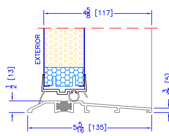
4 5/8" OUTSWING ASSISTED LIVING SILL
