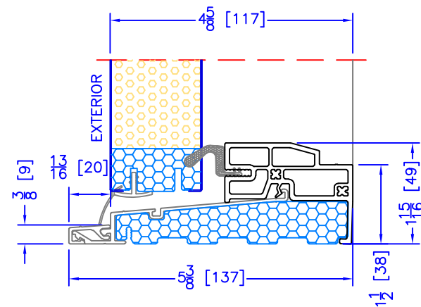
4 5/8" OUTSWING HIGH PERFORMANCE SILL CLOSE-OUT EXTENSION (USED WITH PLAIN FRAME)
