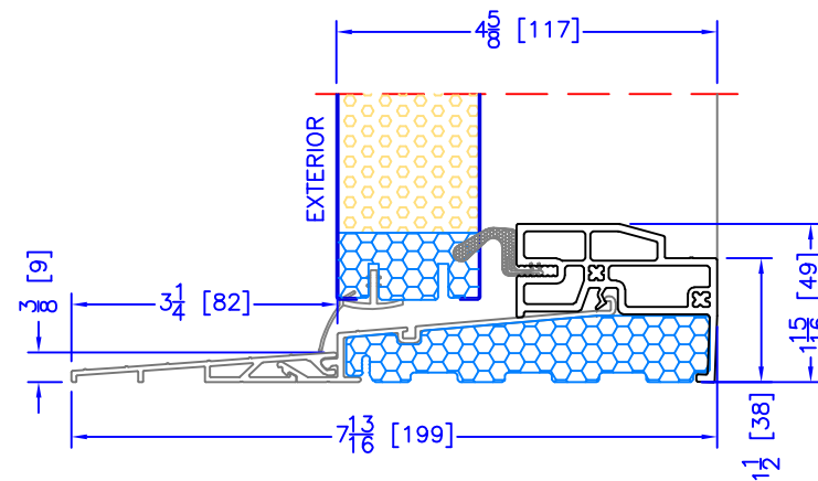
4 5/8" OUTSWING HIGH PERFORMANCE SILL 2 PC ALUMINUM (3/4" EXT) (USED WITH 1 1/2" EXTENDED BM/J-TRIM & FLUSH EXTENSION)
