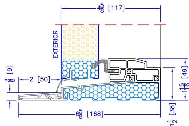
4 5/8" OUTSWING HIGH PERFORMANCE SILL 2 PC ALUMINUM (2" EXT) (USED WITH ALL OTHER EXTERIOR OPTIONS)
