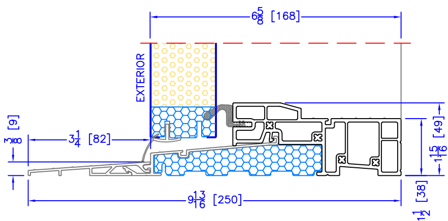
6 5/8" OUTSWING HIGH PERFORMANCE SILL 2 PC ALUMINUM (3/4" EXT) (USED WITH 1 1/2" EXTENDED BM/J-TRIM & FLUSH EXTENSION)
