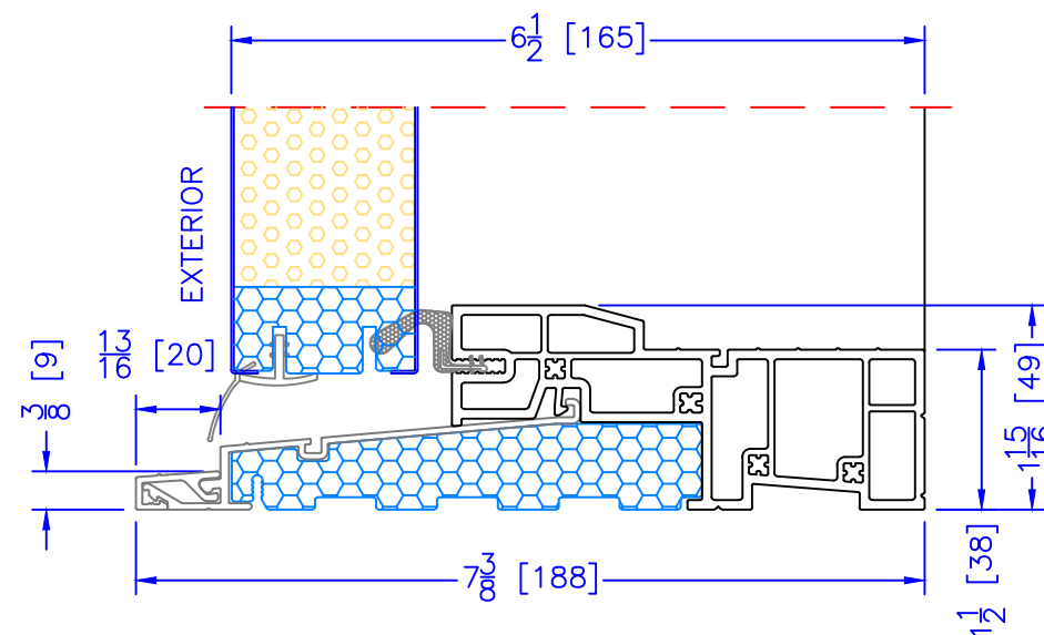
6 1/2" OUTSWING HIGH PERFORMANCE SILL CLOSE-OUT EXTENSION (USED WITH PLAIN FRAME)
