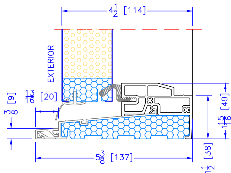
4 1/2" OUTSWING HIGH PERFORMANCE SILL CLOSE-OUT EXTENSION (USED WITH PLAIN FRAME)
