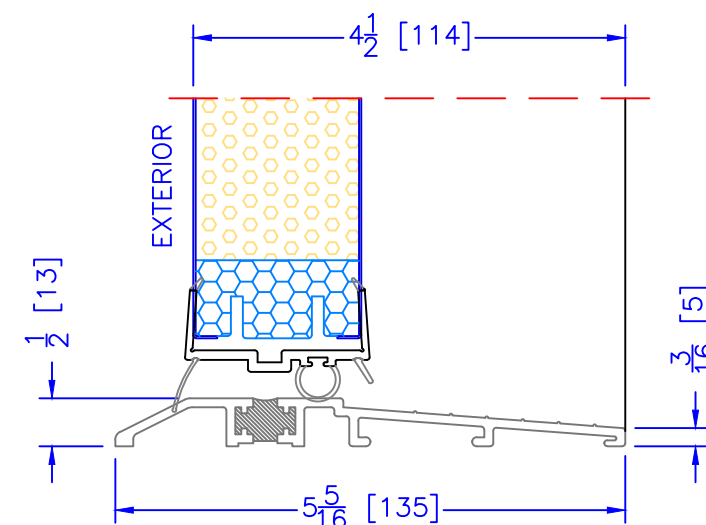
4 1/2" OUTSWING ASSISTED LIVING SILL
