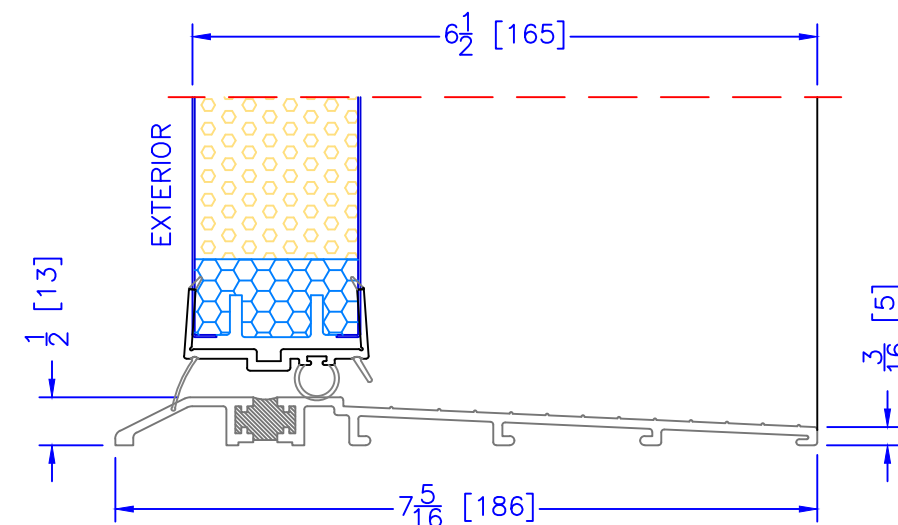
6 1/2" OUTSWING ASSISTED LIVING SILL
