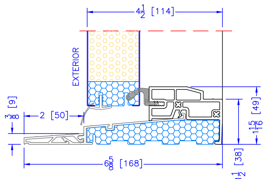
4 1/2" OUTSWING HIGH PERFORMANCE SILL 2 PC ALUMINUM (2" EXT) (USED WITH ALL OTHER EXTERIOR OPTIONS)
