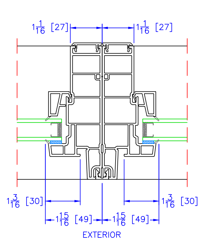
NARROW PICTURE (PN)/NARROW PICTURE (PN) VERTICAL/HORIZONTAL MULLION
