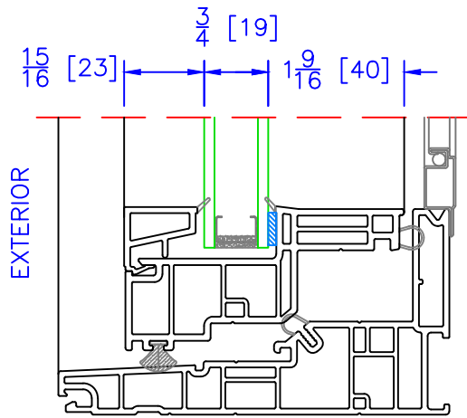
OPERATOR/FIXED DUAL GLAZING OPTION ( \frac{3}{4} " OA)
