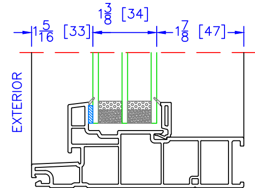
NARROW PICTURE (PN) TRIPLE GLAZING OPTION ( 1\frac{3}{8} " OA)
