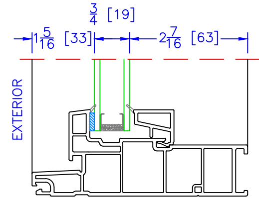
NARROW PICTURE (PN) DUAL GLAZING OPTION ( \frac{3}{4} " OA)
