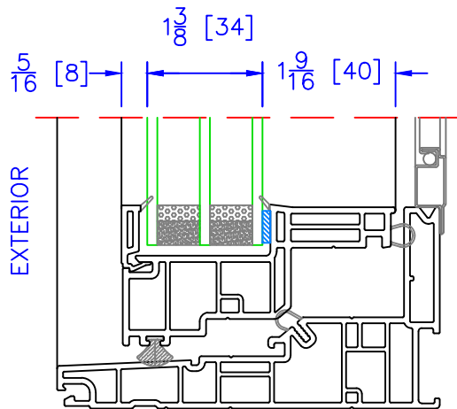
OPERATOR/FIXED TRIPLE GLAZING OPTION ( 1\frac{3}{8} " OA)
