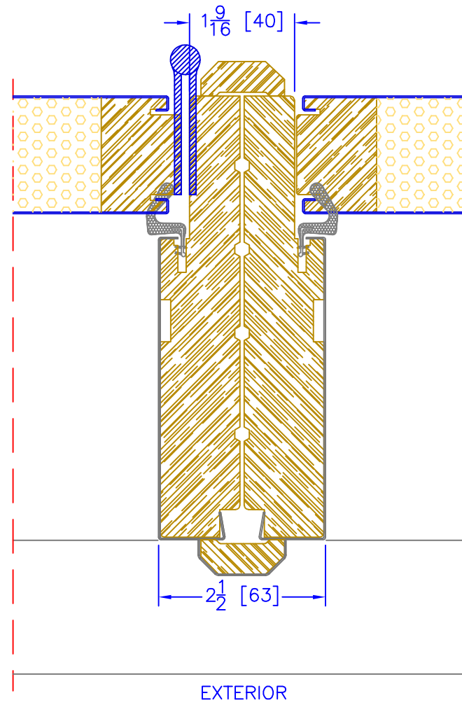
6 5/8" INSWING OPERATOR/SIDELITE VERTICAL MULLION
