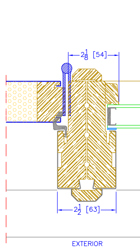
4 5/8" INSWING OPERATOR/S-100 VERTICAL MULLION
