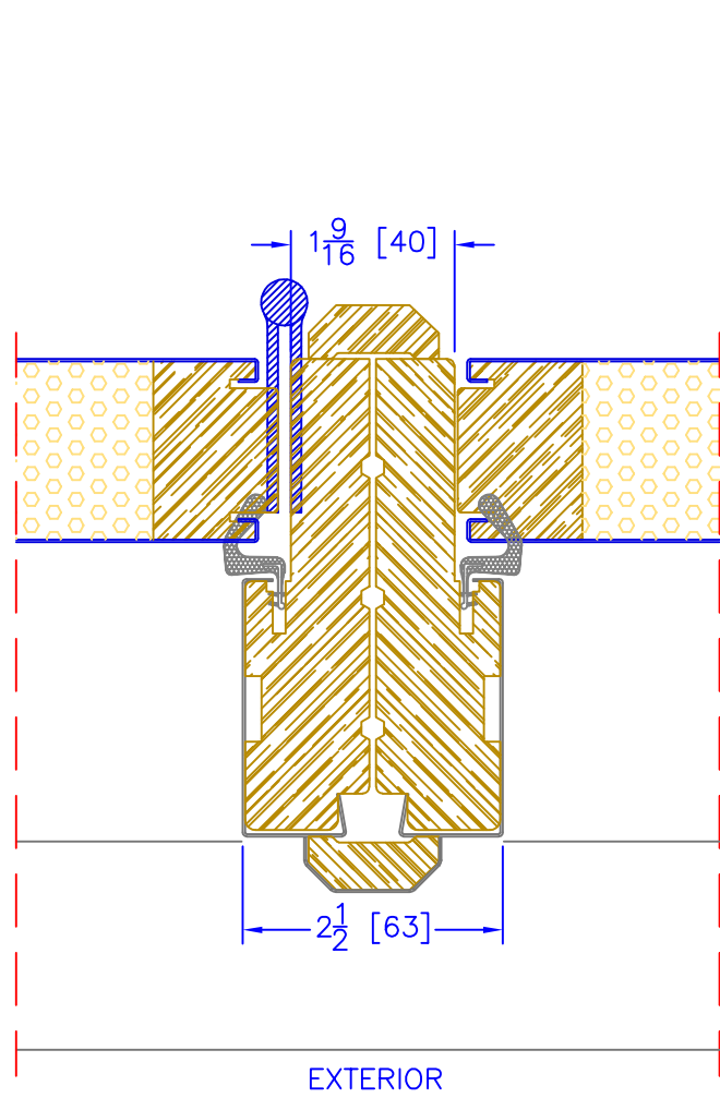
4 5/8" INSWING OPERATOR/SIDELITE VERTICAL MULLION
