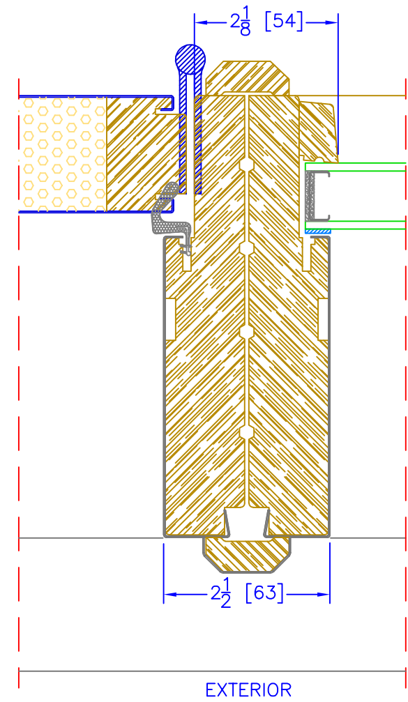
6 5/8" INSWING OPERATOR/S-100 VERTICAL MULLION
