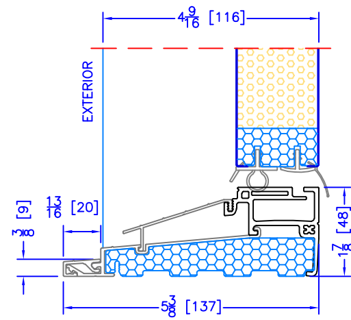
4 7/8" INSWING HIGH PERFORMANCE SILL CLOSE-OUT EXTENSION (USED WITH PLAIN FRAME)
