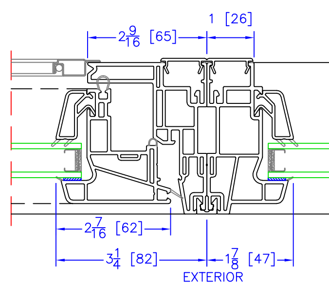
OPERATOR/NARROW PICTURE (PN) VERTICAL/HORIZONTAL MULLION
