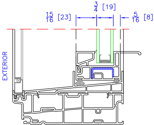
DOUBLE HUNG BOTTOM SASH DUAL GLAZING OPTION ( \frac{3}{4} " OA)
