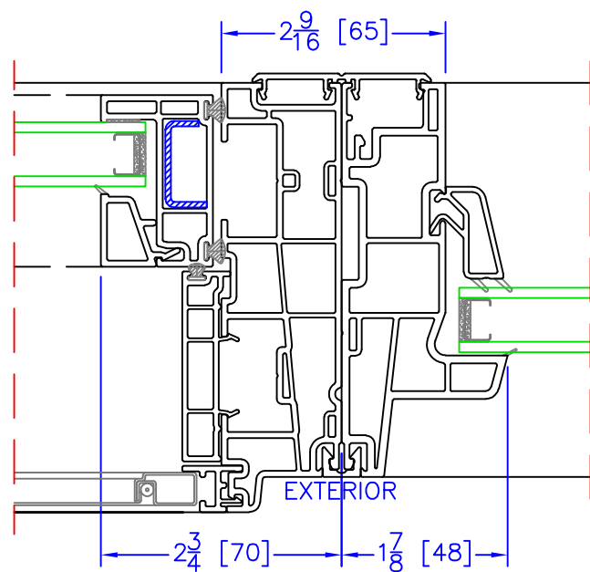
OPERATOR (BOTTOM SASH)/FIXED VERTICAL MULLION
