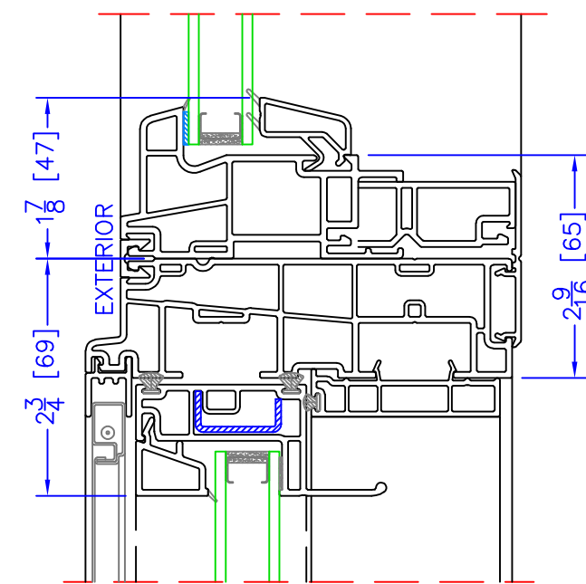
RADIUS SHAPE/OPERATOR HORIZONTAL MULLION
