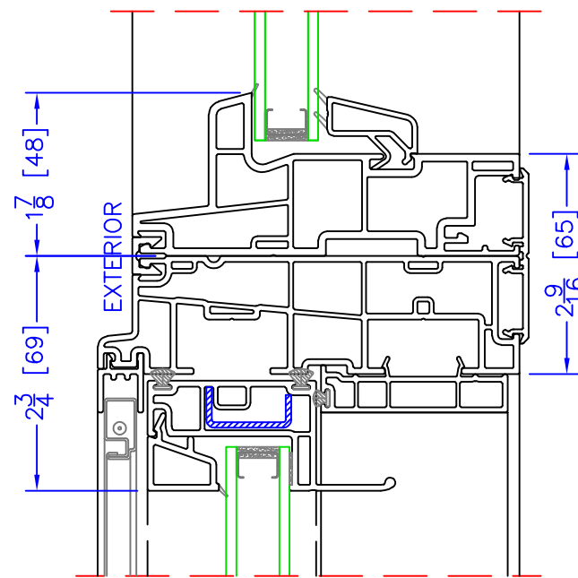
FIXED & POLYGON SHAPE/OPERATOR HORIZONTAL MULLION
