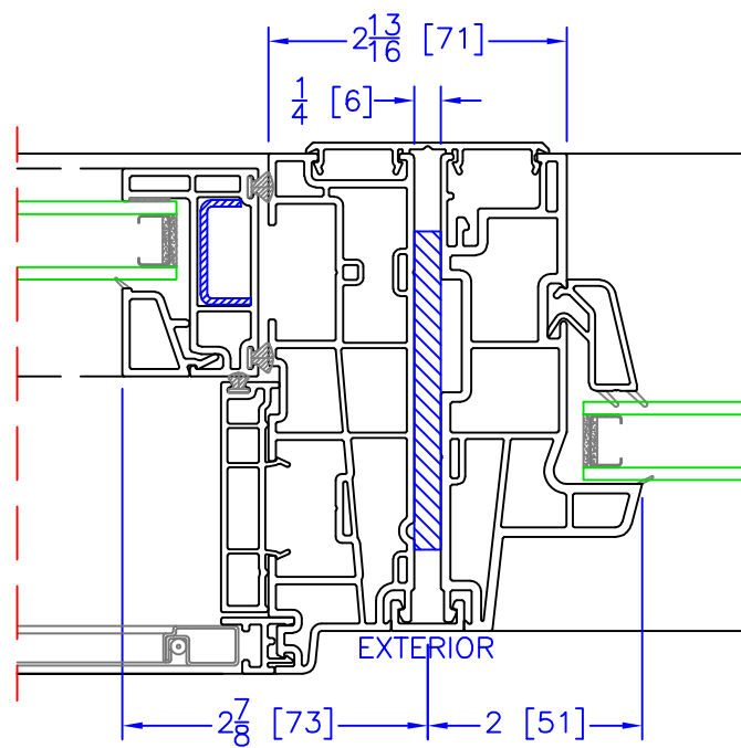
OPERATOR (BOTTOM SASH)/FIXED VERTICAL REINFORCEMENT MULLION
