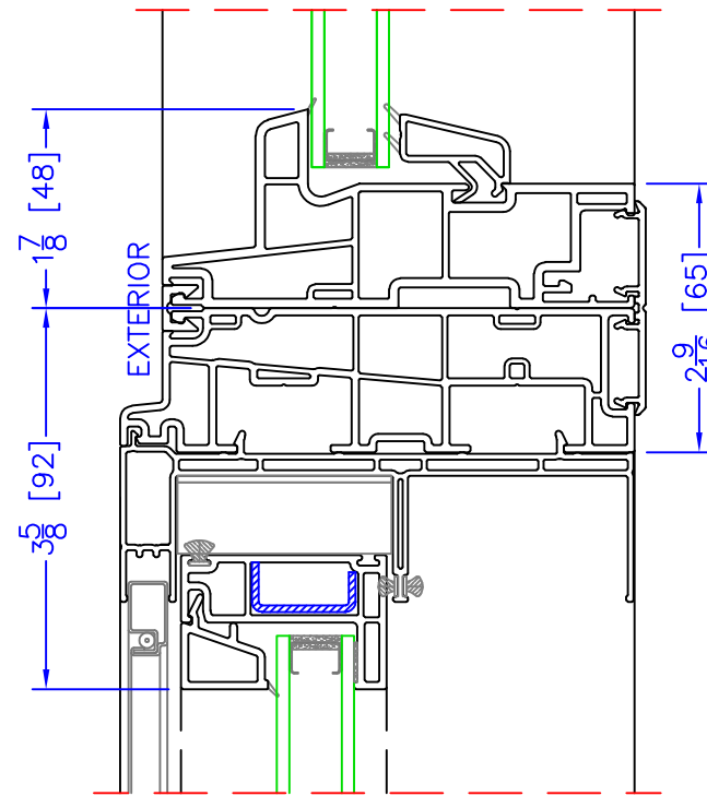
FIXED & POLYGON SHAPE/OPERATOR HORIZONTAL MULLION
