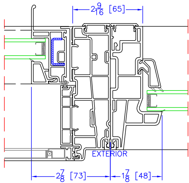
OPERATOR (INSIDE SASH)/FIXED VERTICAL MULLION
