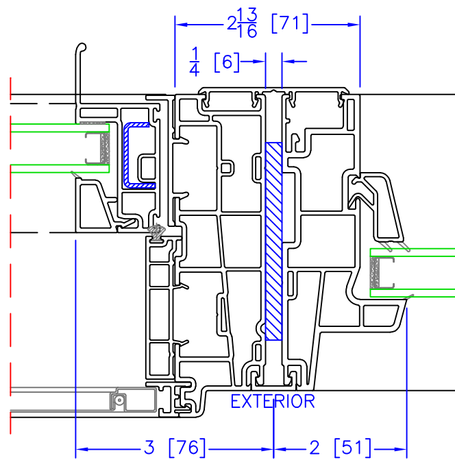
OPERATOR (INSIDE SASH)/FIXED VERTICAL REINFORCEMENT MULLION
