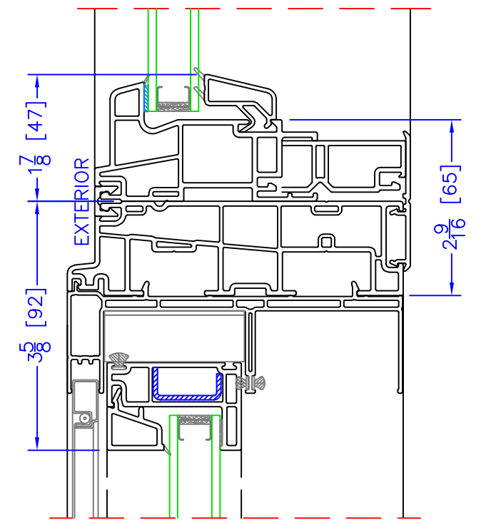
RADIUS SHAPE/OPERATOR HORIZONTAL MULLION
