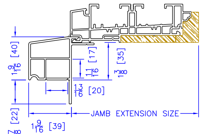
3-1/2" 180 BM/J-TRIM
