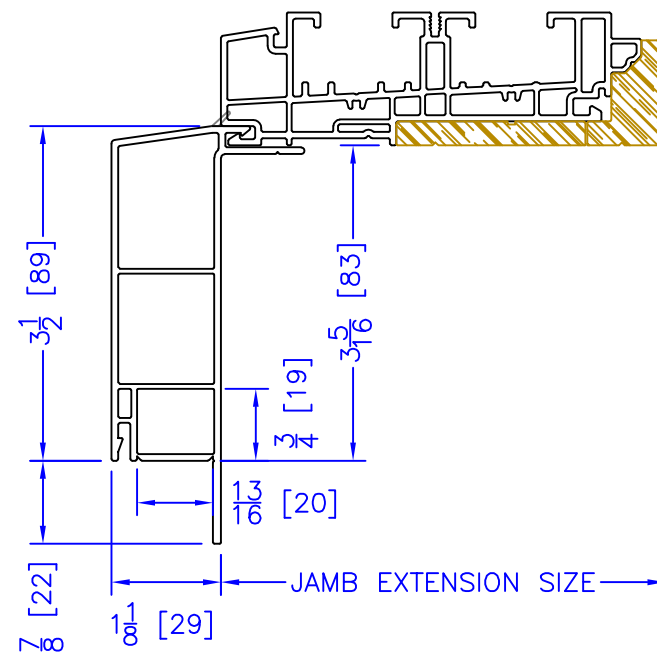
3-1/2" BM/J-TRIM
