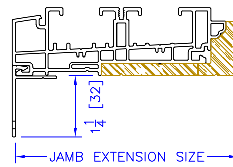
FLASHING FLANGE
