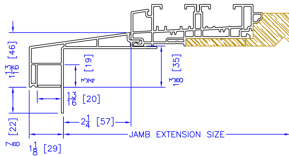
2" 180 BM/J-TRIM
