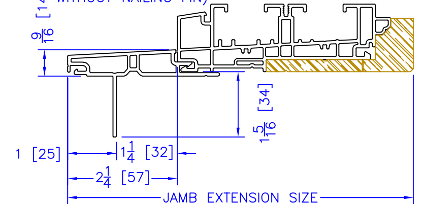
FLUSH EXTENSION (OFFERED WITH AND WITHOUT NAILING FIN)
