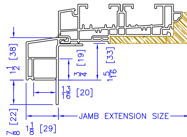
3-1/2" BM/J-TRIM
