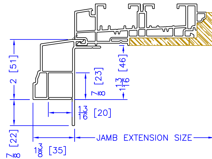
2" 180 BM/J-TRIM
