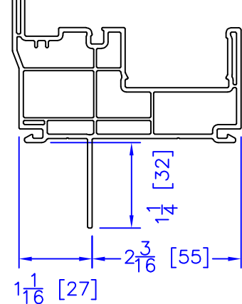
INTEGRAL NAILING FIN
