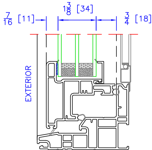
OPERATOR/FIXED TRIPLE GLAZING OPTION ( 1\frac{3}{8} " OA)
