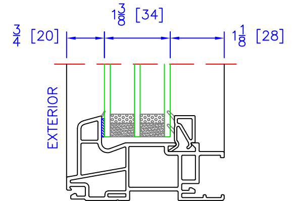
NARROW PICTURE (PN) TRIPLE GLAZING OPTION ( 1\frac{3}{8} " OA)
