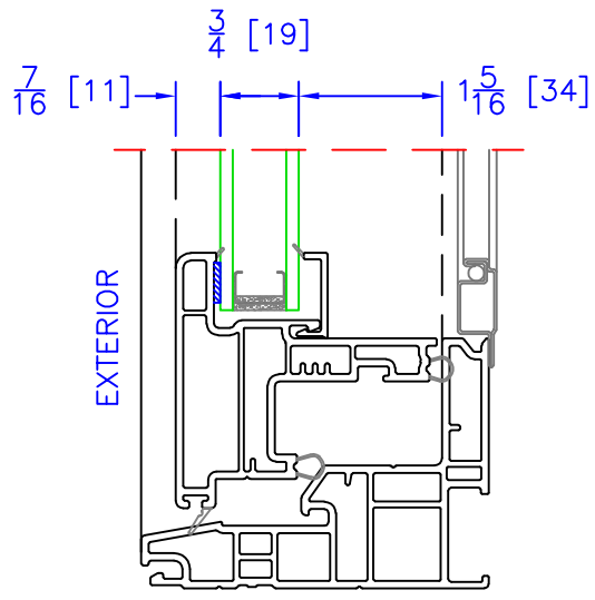
OPERATOR/FIXED DUAL GLAZING OPTION ( \frac{3}{4} " OA)
