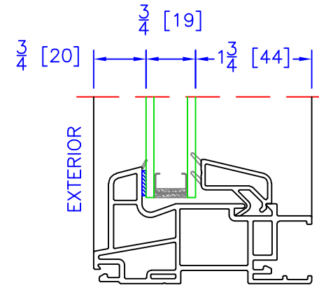
NARROW PICTURE (PN) DUAL GLAZING OPTION ( \frac{3}{4} " OA)
