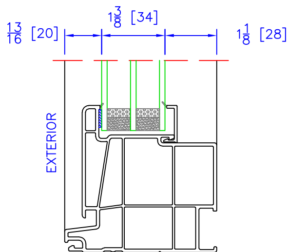
WIDE PICTURE (PW) TRIPLE GLAZING OPTION ( 1\frac{3}{8} " OA)
