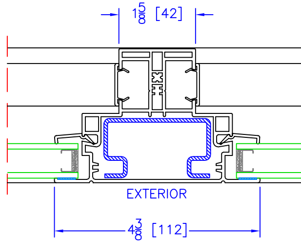
FIXED/FIXED VERTICAL T-MULLION
