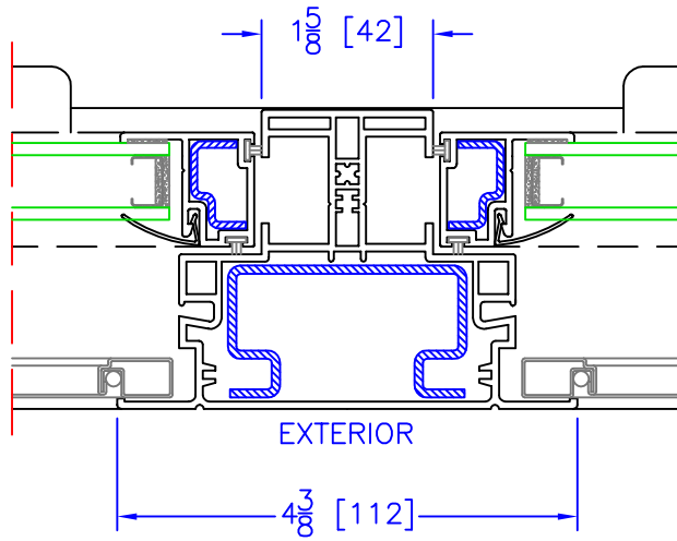
OPERATOR/OPERATOR (BOTTOM SASHES) VERTICAL T-MULLION
