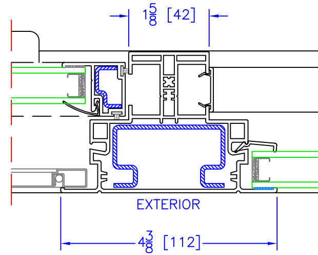
OPERATOR (BOTTOM SASH)/FIXED VERTICAL T-MULLION
