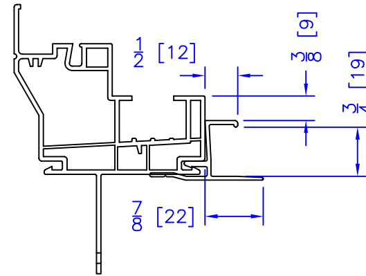
3/4" ADD ON DRYWALL RETURN
