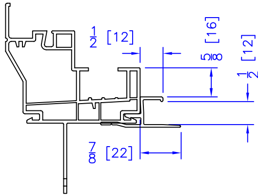
1/2" ADD ON DRYWALL RETURN
