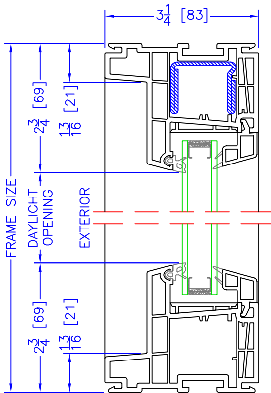
HEAD/SILL
