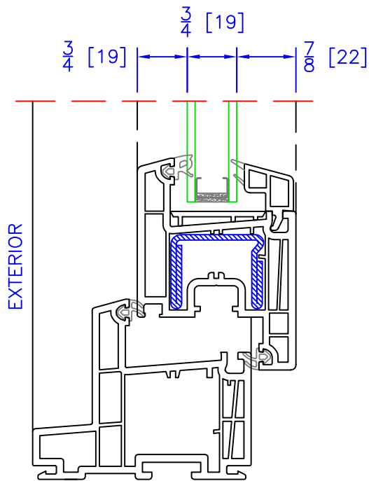
OPERATING/FIXED SASH DUAL GLAZING OPTION (3/4" OA)
