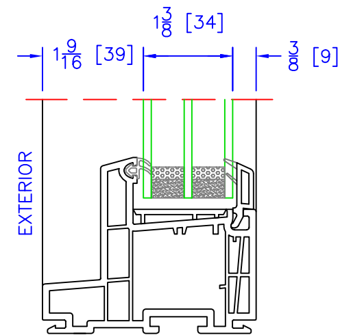
PICTURE WINDOW TRIPLE GLAZING OPTION (13/8" OA)
